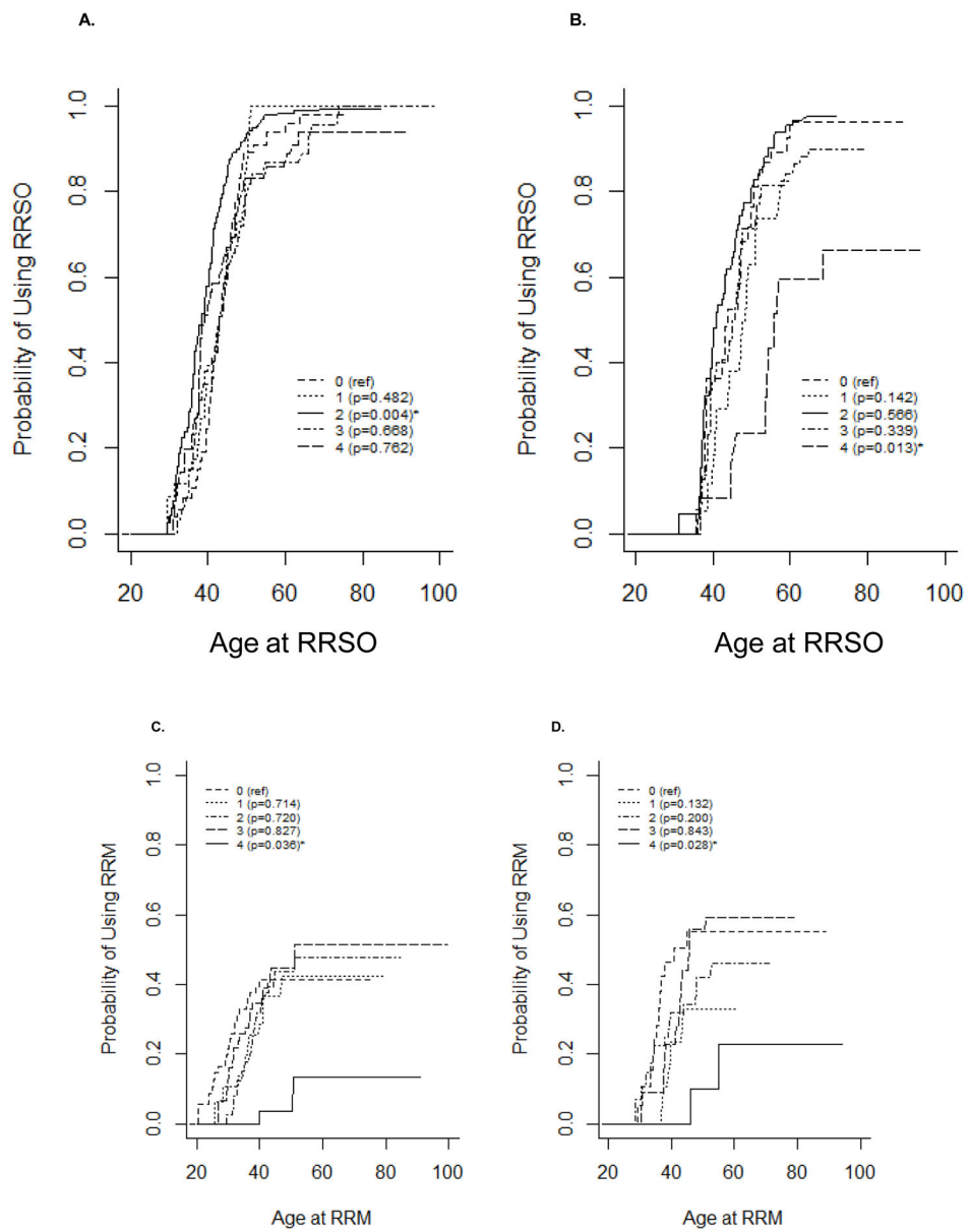
Figure 3. Kaplan-Meier estimates for the cumulative probability of using surgery stratified by the number of live births. A) RRSO-BRCA1; B) RRSO-BRCA2; C) RRM-BRCA1; D) RRM-BRCA2.
