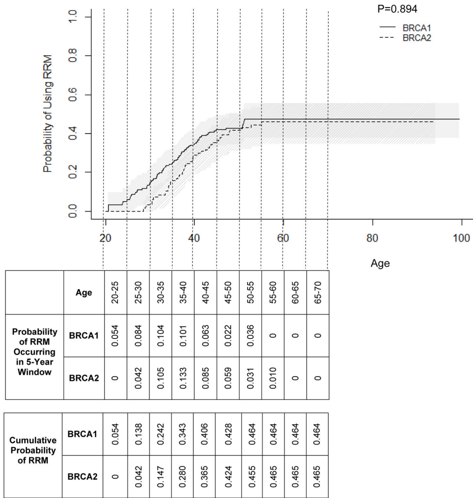
Figure 1. Kaplan-Meier estimates for the cumulative probability of surgery. A) RRSO; B) RRM.
