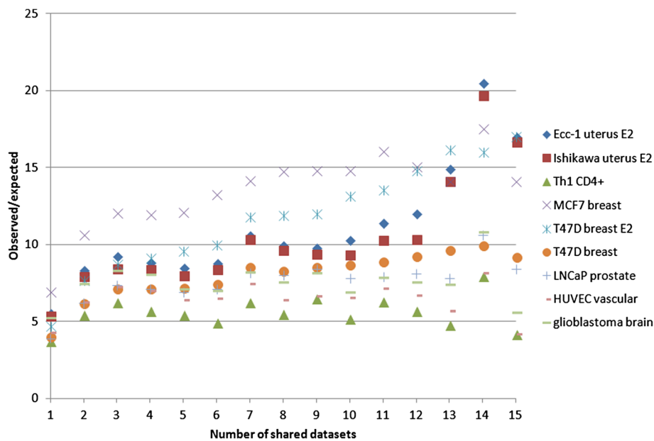
Figure 3 Enrichment of ESR1 binding sites within DNase I hypersensitivity peaks. Different cell types are shown as different series where E2 = estradiol-treated.
