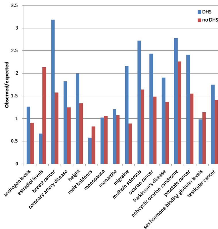
Figure 4 Enrichment of ESR1 binding sites overlapping and not overlapping DNase I hypersensitivity peaks within disease/trait-associated regions. ESR1 binding sites are divided into those overlapping and not overlapping DNase I hypersensitivity peaks in the MCF7 breast cancer cell line.
