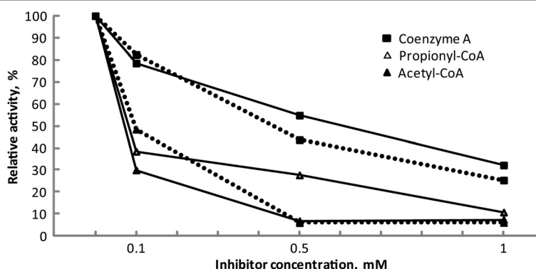
Figure 3 Dependence of the inhibition of FadB' activity on the concentration of acetyl-CoA, propionyl-CoA and CoA. The dotted lines demonstrate the inhibitory effect on FadB' activity measured with acetoacetyl-CoA as substrate. The reaction mixture contained in 100 mM Tris-HCl buffer (pH 7.0) 0.1 mM acetoacetyl-CoA, 0.2 mM NADH, 0.3 \mu\text{g} FadB' Re and the inhibitor CoA or acetyl-CoA at the concentrations as indicated. The straight lines demonstrate the inhibitory effect on FadB' measured with crotonyl-CoA as substrate. The reaction mixture contained in 100 mM Tris-HCl (pH 8.1) 0.1 mM crotonyl-CoA, 2 mM pyruvate, lactate dehydrogenase (9 U), 1.5 mM NAD + , 25 mM MgCl 2 and the inhibitor CoA, acetyl-CoA or propionyl-CoA at the concentrations as indicated. All values are presented as mean values of at least two measurements, standard deviations varied between 0.01% and 3.58%.
