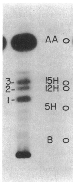
Figure 1. Thin-layer radiochromatogram of human umbilical arterial [1- 14 C]arachidonic acid metabolites. Intact arterial segments (30 mg, dry weight) were incubated with [1- 14 C]arachidonic acid (10 μM) for 30 min in 2 ml of Tris-Hanks'; the metabolites were extracted with chloroform-methanol and analyzed in the hexane-ether-acetic acid system. The positions of reference compounds are indicated. B, PGB 2 ; 5H, 5-HETE; 12H, 12-HETE; 15H, 15-HETE; AA, arachidonic acid.
