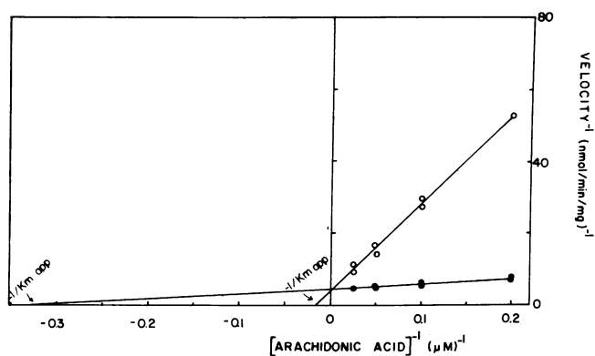
Figure 5. Kinetic analyses of inhibition by 15-HETE of the enzymatic conversion of [ 14 C]arachidonic acid to prostaglandins by cyclooxygenase from human umbilical arterial microsomes. Arterial microsomal protein (400 μg in 500 μl of Tris-GSH) was preincubated in the presence (○) or absence of 15-HETE (100 μM) (●) for 5 min at room temperature. Cyclooxygenase activity was assayed with varying concentrations of [ 14 C]arachidonic acid (5–40 μM) at 37°C for 5 min. Cyclooxygenase activity is expressed as the sum of 6kPGF 1α , PGE 2 , and PGF 2α production (no PGI 2 , TXB 2 , or PGD 2 was detected in these experiments). Lineweaver–Burk plots were generated using linear regression analyses.
