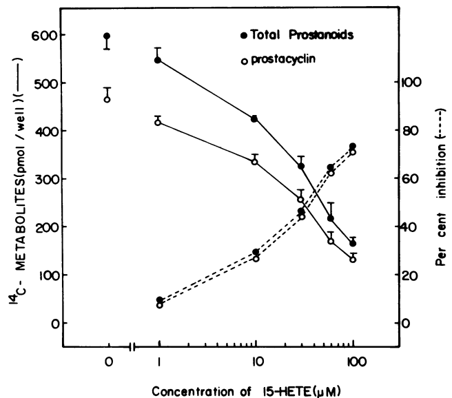
Figure 8. Concentration-dependent inhibition by 15-HETE of the conversion of exogenous [1- 14 C]arachidonic acid to prostaglandins. Fetal bovine aortic endothelial cell monolayers were preincubated for 15 min with the indicated concentrations of 15-HETE (1–100 μM), in 750 μl of MEM. [1- 14 C]arachidonic (5 μM) was then added and the incubation was continued for a further 60 min. The products were extracted in chloroform-methanol as previously described and analyzed by TLC radioautography-liquid scintillation counting. Values represent the mean ± 1 SD of four different experiments. Total prostacyclin is sum of 6kPGF 1α and PGI 2 production. Total prostanoids are sum of 6kPGF 1α , PGF 2α , PGE 2α , PGI 2 , and TXB 2 production. No PGD 2 was detected in these experiments.
