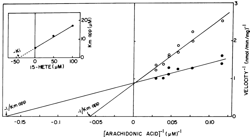
Figure 9. Kinetic analyses of inhibition by 15-HETE of the enzymatic conversion of [1-^{14}\text{C}] arachidonic acid to prostaglandins by cyclooxygenase from endothelial cell microsomes. Endothelial cell microsomal protein (250 \mu\text{g} in 500 \mu\text{l} of Tris-GSH) was preincubated in the presence (○) or absence (●) of 15-HETE (100 \mu\text{M} ) for 5 min at room temperature. Cyclooxygenase activity was assayed with varying concentrations of [1-^{14}\text{C}] arachidonic acid (8.6–34.5 \mu\text{M} ) at 37°C for 5 min. Cyclooxygenase activity is expressed as the sum of 6kPGF 1 \alpha , PGE 2 , TXB 2 , and PGF 2 \alpha production (no PGD 2 or PGI 2 was detected in these experiments). Lineweaver-Burk plots were generated using linear regression analyses. (Inset) K_m apparent from experiments at 0, 50, and 100 \mu\text{M} 15-HETE were calculated and K_i determined from linear regression analysis of a Dixon plot.
