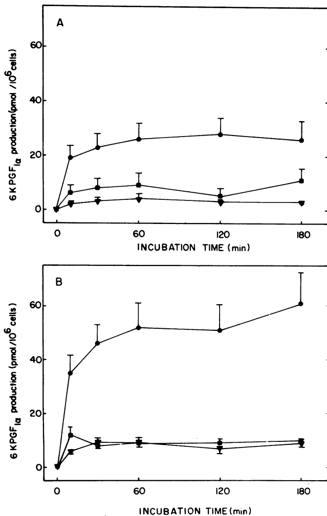
Figure 7. Effect of 15-HETE on basal and bradykinin-stimulated release of immunoreactive 6kPGF 1α . Fetal bovine aortic endothelial cells were incubated in the presence or absence of varying concentrations of 15-HETE in 1.0 ml of MEM. Aliquots of cell culture media were removed at indicated times and assayed for 6kPGF 1α content by RIA. At the end of the experiment, cells were trypsinized and counted. Values are the mean ± 1 SE of four different experiments corrected for cross-reactivity of 15-HETE at zero time. (A) Basal release of 6kPGF 1α ; (B) bradykinin (10 μg/ml)-stimulated release of 6kPGF 1α . (●) Control; (■) 50 μM 15-HETE; (▼) 100 μM 15-HETE.
