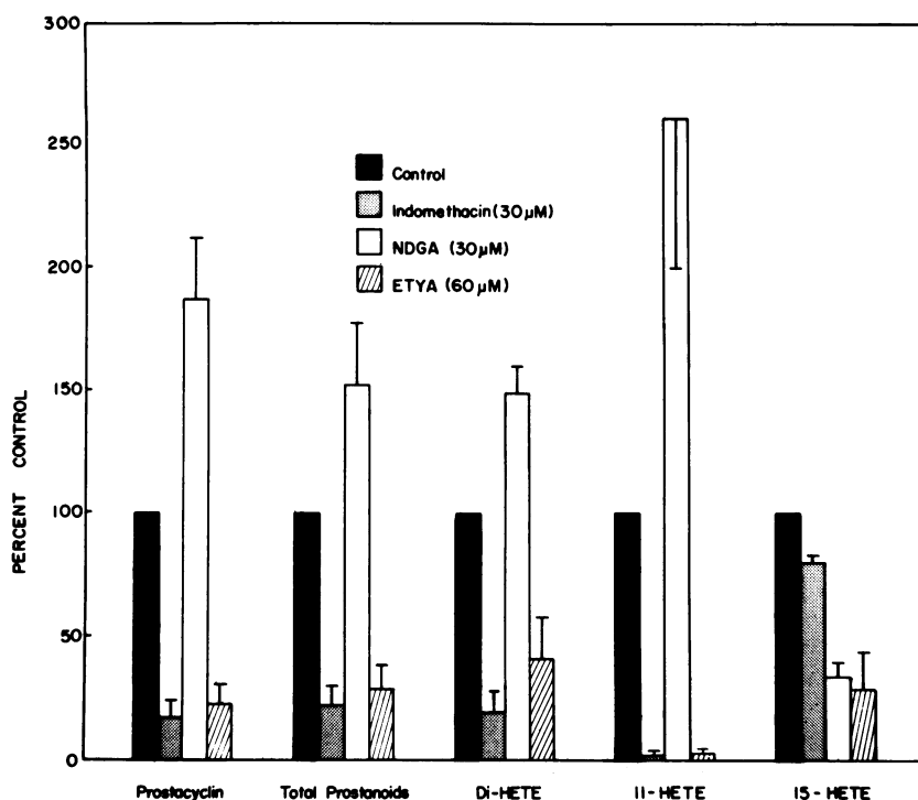
Figure 3. Effect of indomethacin, NDGA, and ETYA on [1-^{14}\text{C}] arachidonic acid metabolism by human umbilical arteries. Intact arterial segments (20–30 mg, dry weight) were preincubated at 37^\circ\text{C} for 10 min in 2 ml of Tris-Hanks' alone or containing indomethacin ( 30\ \mu\text{M} ), NDGA ( 30\ \mu\text{M} ), or ETYA ( 60\ \mu\text{M} ). [1-^{14}\text{C}] Arachidonic acid ( 10\ \mu\text{M} ) was then added, and the incubation was continued for a further 30 min. The products were analyzed as described in Methods. Values represent the mean \pm 1 SE of five experiments. Total prostanoids are the sum of 6\text{kPGF}_{1\alpha} , \text{PGF}_{2\alpha} , \text{PGE}_2 , \text{TXB}_2 , and \text{PGI}_2 production. Total prostacyclin is the sum of 6\text{kPGF}_{1\alpha} and \text{PGI}_2 production.
