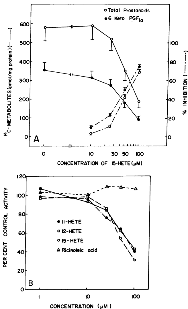
Figure 4. Concentration-dependent inhibition of human umbilical arterial microsomal cyclooxygenase by HETEs. Human umbilical arterial microsomes (500 μg in 500 μl of Tris-GSH) were preincubated with the indicated concentrations of HETEs (1–100 μM) for 5 min at room temperature. The cyclooxygenase reaction was initiated by addition of [ 14 C]arachidonic acid (10 μM) and terminated after 10 min. The products were analyzed by TLC radioautography–liquid scintillation countings. Total prostanoids are sum of 6kPGF 1α , PGF 2α , and PGE 2 production (no PGD 2 , TXB 2 , or PGI 2 was detected in these experiments). (A) Effect of 15-HETE (10–100 μM) on total prostanoids and 6kPGF 1α production. Values represent the mean ± 1 SE of four different experiments each performed in duplicate. (B) Effect of 11-HETE, 12-HETE, 15-HETE, and ricinoleic acid (1–100 μM) on total prostanoids and 6kPGF 1α production. Results depicted are from a representative experiment.
