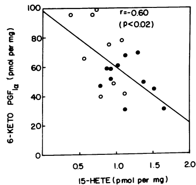
Figure 6. Evaluation of 15-HETE and 6kPGF 1α release by normal and diabetic human umbilical arteries. Umbilical arterial segments were incubated in Tris-Hanks' at 37°C for 30 min, and the medium was assayed for 15-HETE and 6kPGF 1α content by RIA. Values represent product released in picomoles per milligram of tissue dry weight. (●) Diabetic tissues; (○) normal tissues. The correlation coefficient was determined using linear regression analysis.
