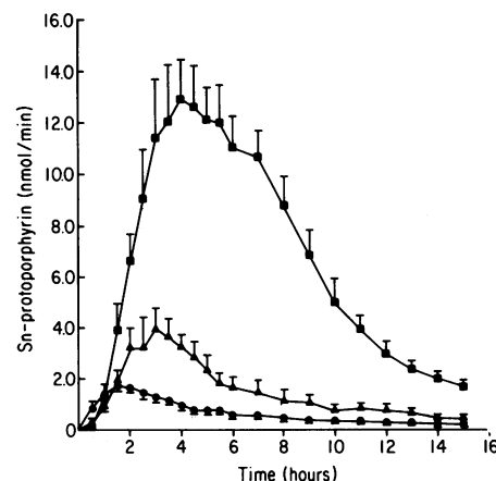
Figure 5. Excretion of Sn-protoporphyrin in bile in bile duct-cannulated rats. Three groups of rats were treated with single doses of 10 μmol/kg bw i.v. (eight rats, circles), 20 μmol/kg bw subcutaneously (three rats, triangles) or 50 μmol/kg bw subcutaneously (four rats, squares). Values shown are mean±SE for each group. See text for details.
