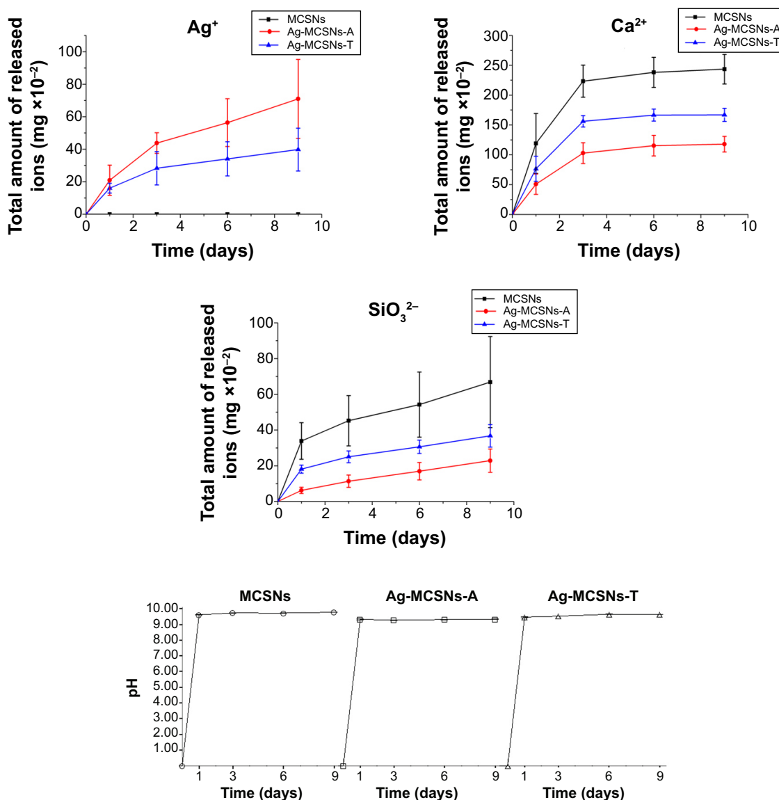
Figure 4 Ag + , Ca 2+ , and SiO 3 2- ion release profile and pH measurement of MCSNs, Ag-MCSNs-A, and Ag-MCSNs-T over time.
