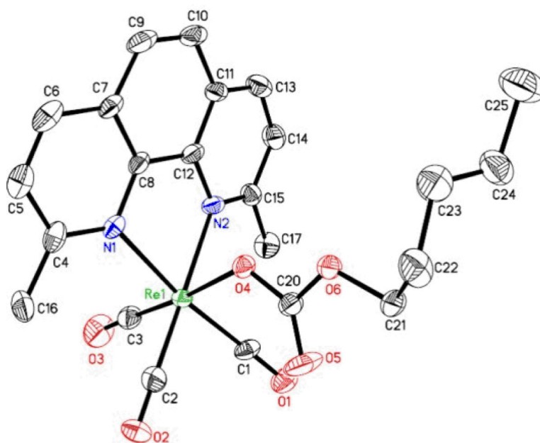
Fig. 2. X-ray structure of PC 4
