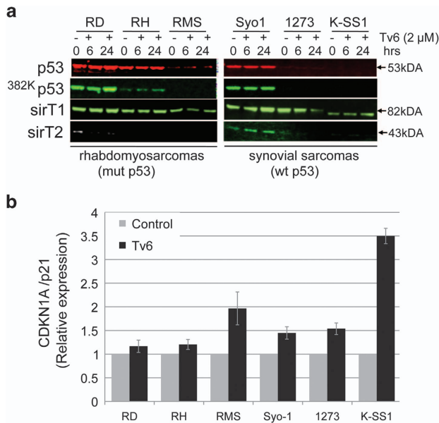
Figure 3 Tenovin-6 induces p21 expression without affecting p53 acetylation at lysine 382. (a) Expression of p53 and acetylated p53 ( Ac 382K p53). Cells were incubated with 2 μM Tv6, and total protein extracts from the cells were collected after 6 and 24 h for western blot using specific antibodies and infrared conjugates (IR-dye conjugates), and visualized simultaneously using the Odyssey system. (b) CDKN1A/p21 expression in Tv6-treated and control cells determined by QRT-PCR. Relative expression in relation to GAPDH is shown
