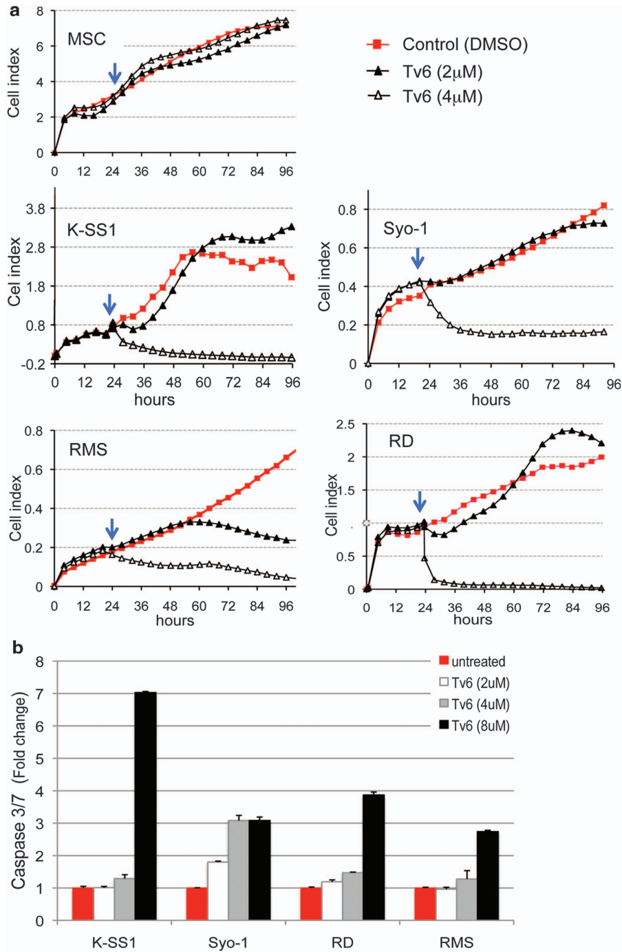
Figure 2 The sirtuin inhibitor tenovin-6 inhibits cell proliferation and induces caspase 3/7 activity in pediatric soft tissue sarcomas. (a) Cell proliferation curves of control and tenovin-6 (Tv6)-treated soft tissue sarcoma cell lines followed in real time over a 96-h period using the xCELLigence bioanalyzer. Cells were plated and allowed to form monolayers. The drug was added 24 h after plating (blue arrow). Cell index is a relative unit derived from changes in electrical impedance in a surface; in this case, impedance is proportional to cell confluence giving a quantitative rate of cell numbers. (b) Caspase 3/7 activity was measured in cells after 48 h treatment with Tv6. The fold change is relative to untreated control cells (value = 1). Syo-1 and K-SS1: synovial sarcoma cell lines. RD: embryonal rhabdomyosarcoma. RMS: alveolar rhabdomyosarcoma. MSC: mesenchymal stem cells
