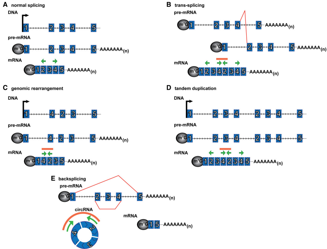
FIGURE 5. Scrambled exon junctions can be formed from different mechanisms. Outward-facing primers in exons 2 and 4 (green arrows) will not yield an RT-PCR product if the exons are ordered linearly (A), but will yield a product, indicated by orange line above primers, if the exons are scrambled in the mRNA. Scrambled exons could occur through trans -splicing (B), genomic rearrangements (C), including tandem duplication within the DNA (D), or backsplicing (E). (Red lines) Unusual (nonsequential) splicing, (arrowheads) 5'–3' direction, (green arrows) outward-facing PCR primers, and (orange line) RT-PCR product.
