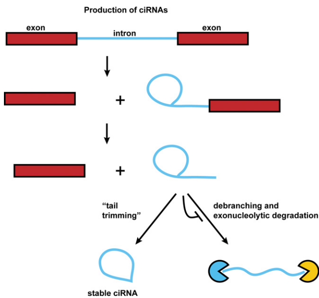
FIGURE 2. Production of ciRNAs. Circular intronic RNAs are produced by eukaryotic spliceosome-mediated splicing. The lariat intron generated from the splicing reaction evades normal debranching and degradation, and instead the 3' "tail" downstream from the branchpoint is trimmed resulting in a stable ciRNA.
