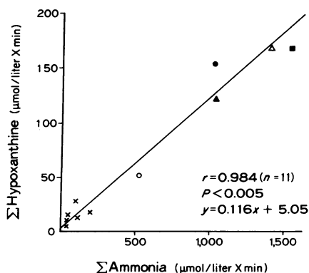
Figure 6. Relation of the incremental area of venous ammonia ( \Sigma ammonia) to that of hypoxanthine ( \Sigma hypoxanthine) in the forearm exercise tests. Data from Table II were used: control subjects (x), patient 1 (●), patient 2 (○), patient 3 (▲), patient 4 (△), and patient 5 (■).
