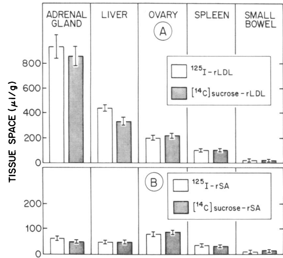
Figure 2. Comparison of the tissue spaces achieved by rLDL and rSA in the liver and various extrahepatic tissues when labeled with either [ ^{14}\text{C} ]sucrose or ^{125}\text{I} . Groups of rats were killed 10 min after the intravenous administration of either [ ^{14}\text{C} ]sucrose-rLDL, ^{125}\text{I} -rLDL, [ ^{14}\text{C} ]sucrose-rSA, or ^{125}\text{I} -rSA, and the space achieved by each protein in 15 tissues, only five of which are shown, was determined. Each value represents the mean \pm 1 SEM of data obtained in six animals.
