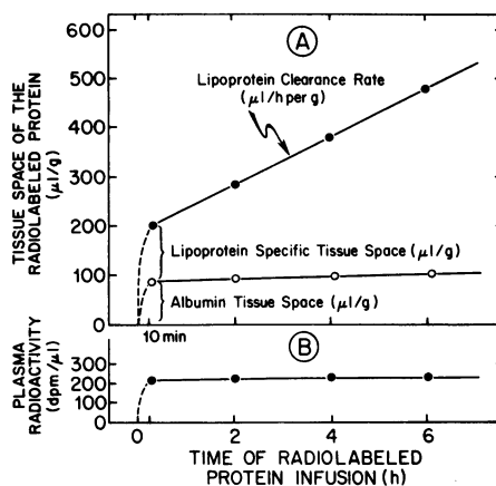
Figure 1. Diagrammatic representation of the protocol used in measuring the specific tissue space and clearance rate of labeled lipoproteins by the various tissues of the rat. As shown in B, a bolus of radiolabeled protein was administered intravenously at time zero, and was followed by a constant infusion of the same radiolabeled preparation for varying periods up to 6 h. Using the measured whole animal plasma clearance rate of each lipoprotein preparation, the amount of radioactivity infused per hour was adjusted relative to the dose given as a bolus in order to maintain the specific activity of the radiolabeled protein in the plasma at a constant level throughout the period of infusion. As shown in A, groups of animals were then killed at 10 min, 2 h, 4 h, and 6 h, and the plasma and 15 tissues were assayed for radioactive content. The radioactivity present in 1 g of each organ (dpm/g) was divided by the concentration of radiolabeled protein in the plasma (dpm/ \mu l) to give the space of distribution achieved by each radiolabeled compound at each time point. The slope of the linear regression curves fitted to these values gives the rate of tissue uptake of the various test molecules expressed as the microliter of plasma cleared of its content of LDL or methyl-LDL each hour by 1 g of tissue. In A, typical curves are shown for a tissuelike liver in animals infused with either rLDL (●) or rSA (○).
