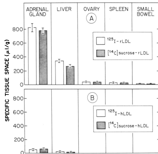
Figure 3. Comparison of the specific tissue spaces achieved by rLDL and hLDL in the liver and various extrahepatic tissues when labeled with either [ ^{14}\text{C} ]sucrose or ^{125}\text{I} . Groups of rats were killed 10 min after the intravenous administration of either [ ^{14}\text{C} ]sucrose-rLDL, ^{125}\text{I} -rLDL, [ ^{14}\text{C} ]sucrose-hLDL, or ^{125}\text{I} -hLDL, and the specific tissue space achieved by each protein in 15 tissues, only five of which are shown, was determined. Each value represents the mean \pm 1 SEM of data obtained in six animals.
