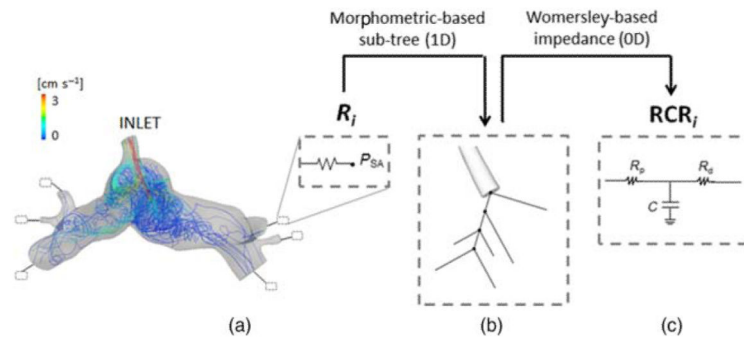
Figure 3. Pre-operative pulmonary LPM generation. A resistance R_i is computed for each i th outlet of the 3D model (a) by means of steady simulations (velocity-colored pathlines are displayed); R_i is first converted in a morphometric-based sub-tree (b), then in the corresponding Womersley-based impedance RCR_i (c). P_{SA} = single atrium pressure; R_p = proximal resistance; R_d = distal resistance; C = compliance.
