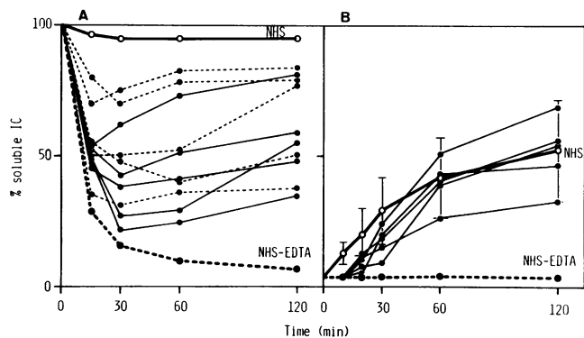
Figure 1. (A) IIP of ^{125}\text{I} -BSA-anti-BSA antibody complexes in various sera. The initial reaction mixture containing 0.5 \mu\text{g} ^{125}\text{I} -BSA and 50 ml serum was diluted to a final volume of 120 \mu\text{l} with CFD buffer, and incubated for 5 min at 37^\circ\text{C} . 9 mg of rabbit anti-BSA antibody was added and the incubation was continued at 37^\circ\text{C} . At various time intervals, 25- \mu\text{l} aliquots were removed, mixed with 1 ml of cold PBS buffer, and centrifuged for 15 min at 3,000 g . After separation of pellet and supernatant, the percentage of soluble complexes was determined. NHS: (— \circ —); NHS chelated with 10 mM EDTA (NHS-EDTA): (--- \bullet ---). Patients of group A of the table: patients 3-7 (uterine myoma, paraproteinemia): (— \bullet —) patients 8-12 (cryoglobulinemia): (--- \bullet ---). (B) SOL of ^{125}\text{I} -BSA-anti-BSA aggregates in different sera. Preformed immune aggregates (1.9 \mu\text{g} ) were incubated at 37^\circ\text{C} with 50 \mu\text{l} test serum in a final volume of 120 \mu\text{l} . SOL \pm 2 SD in normal human serum are indicated: (— \circ —). Patients with early classical pathway depletion (patients 3-7): (— \bullet —).
