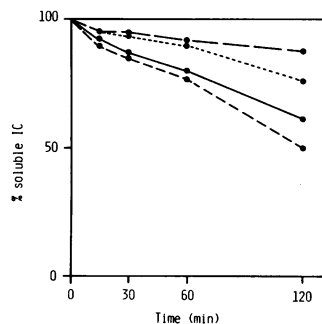
Figure 3. IIP in the four sera of patients with C3 depletion (patients 16-19). Patients: 16: (— \bullet —); 17: (--- \bullet ---); 18: (— \circ —); 19: (--- \circ ---).
