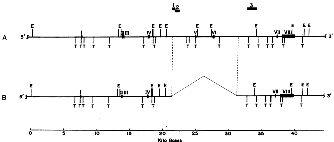
Figure 5. The site of the deletion in the abnormal factor IX gene. A shows the normal factor IX gene with Eco R1 ( E ) and Taq I ( T ) sites. Exons are shown as solid regions labeled with roman numerals (I to VIII). The sites of the genomic probes employed are depicted as solid bars with arabic numbers at the top (1 to 3). B shows the factor IX
