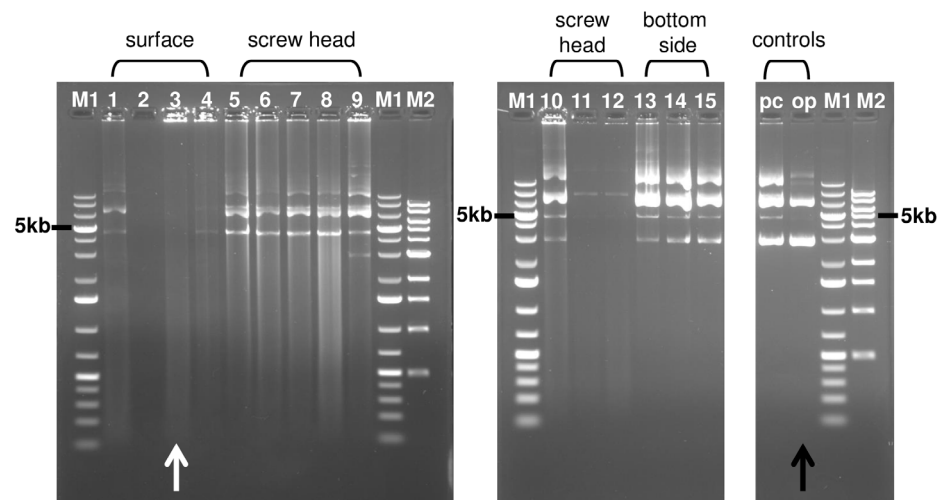
Figure 4. DNA quality analysis by agarose gel electrophoresis. For each sample 250 ng of DNA was loaded on an agarose gel and the degree of degradation was analyzed after the run. The highest degree of degradation was recorded for samples 1–4, which were applied directly to the surface of the payload. For the samples applied in the grooves of the screw heads a lower degree of degradation was observed. DNA with the highest integrity was observed for the samples applied on the bottom side of the payload. The white arrow depicts the sample with the highest degree of degradation. The black arrow points to the lane where the original plasmid (op) was loaded. M1: Marker Gene Ruler 1 kb ladder; M2: Marker 1 kb DNA ladder; pc: positive control (9 days ground control).
