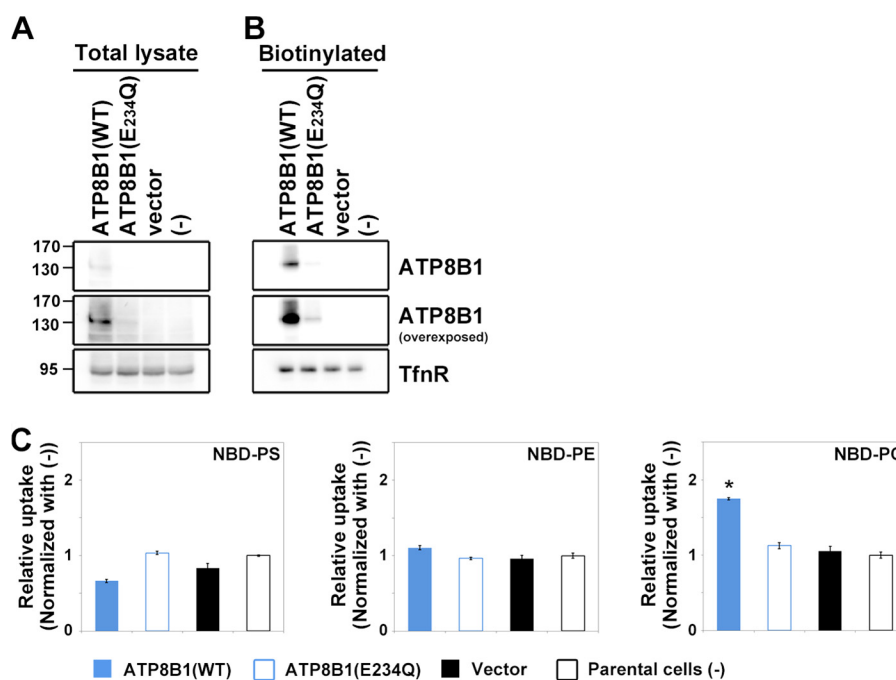
FIGURE 7. Flippase activity of ATP8B1 across the leaflets of the plasma membrane in CHO-K1 cells. CHO-K1 cell lines stably expressing HA-tagged ATP8B1(WT) or ATP8B1(E234Q) were established by infection with recombinant retrovirus followed by selection in the presence of antibiotics. A , the total expression level of ATP8B1 was analyzed by immunoblotting with antibodies against HA and TfnR (as an internal control). 4% of the input of the biotinylation reaction was loaded in each lane. B , the cell surface expression level of ATP8B1 was determined by surface biotinylation analysis. The middle panels show overexposures. C , cells were incubated with NBD-lipids and processed for flippase assays as described in the legend for Fig. 4. -Fold increase of NBD-lipid uptake relative to parental CHO-K1 cells (-) is shown. The results display averages from triplicates \pm S.D. (*, p < 0.001 ). Error bars represent S.D.
