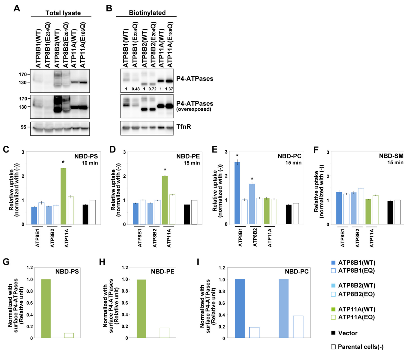
FIGURE 5. Cell surface expression and flippase activities of P4-ATPases in retrovirus-infected HeLa stable cells. HeLa cells stably expressing the indicated HA-tagged P4-ATPases were established by infection with recombinant retrovirus without clonal selection and processed for analysis of the total (A) or cell surface (B) expression level of the P4-ATPase proteins as described in the legend for Fig. 3. The middle panels of A and B show overexposures of the blots shown in the top panels. Cells expressing ATP8B1, ATP8B2, and ATP11A were incubated with NBD-PS (C), NBD-PE (D), NBD-PC (E), or NBD-SM (F) at 15 °C for 15 min (or 10 min for NBD-PS). After extraction with fatty acid-free BSA, the residual fluorescence intensity associated with the cells was determined by flow cytometry. -Fold increase of NBD-lipid uptake relative to parental HeLa cells (-) is shown. The graphs are representative of two independent experiments, and results display averages from triplicates \pm S.D. (*, p < 0.001 ). Error bars represent S.D. G-I, the enzymatic activities were normalized with the level of biotinylated P4-ATPases shown in B.
