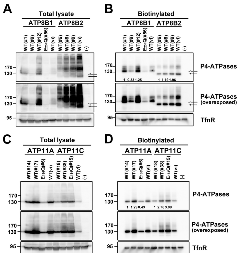
FIGURE 3. Cell surface expression of P4-ATPases in HeLa stable cell lines. HeLa cell lines stably expressing HA-tagged P4-ATPase were established by plasmid transfection followed by selection in the presence of antibiotics. Two or three independent clones of cells expressing ATP8B1(WT), ATP8B2(WT), ATP11A(WT), or ATP11C(WT) or one clone expressing ATP8B1(E234Q), ATP11A(E186Q), or ATP11C(E184Q) was examined. A and C , the total expression level of the P4-ATPase in each cell line was analyzed by immunoblotting with anti-HA and anti-TfnR antibodies (as an internal control). 4% of the input of the biotinylation reaction was loaded in each lane. Arrow , ATP8B2; open arrow , ATP8B1. B and D , the cell surface level of the P4-ATPase in each cell line was analyzed after surface biotinylation. Proteins precipitated with streptavidin-agarose beads were subjected to immunoblot analysis for HA and TfnR (as an internal control). The numbers show the relative expression level of proteins, which were normalized with the level of the internal control, TfnR, and were used for normalizing the enzymatic activities shown in Fig. 4 ( J and K ). In A–D , open and solid arrows indicate positions of ATP8B1 and ATP8B2, respectively. In A–D , middle panels show overexposures. WT(vi) , cell lines established by infection of recombinant retrovirus for each P4-ATPase.
