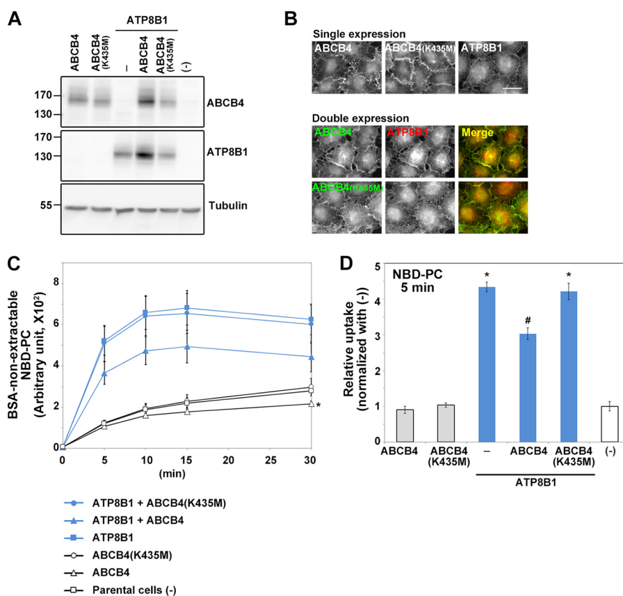
FIGURE 9. Exogenous expression of ABCB4 antagonizes PC flipping mediated by ATP8B1. HeLa cell lines stably expressing HA-tagged ATP8B1, FLAG-tagged ABCB4(WT), FLAG-tagged ABCB4(K435M), ATP8B1-HA + FLAG-ABCB4(WT), or ATP8B1-HA + FLAG-ABCB4(K435M) were established by infection with recombinant retroviral vectors. A , the total expression level of each protein was analyzed by immunoblotting with anti-HA, anti-DYKDDDDK (which recognizes the FLAG epitope), and anti- \beta -tubulin antibodies. B , cells expressing the indicated proteins singly or doubly were processed for immunostaining with anti-HA and anti-DYKDDDDK antibodies followed by Cy3-conjugated anti-rat and DyLight649-conjugated anti-mouse secondary antibodies. Scale bar, 20 \mu m. C , cells were incubated with NBD-PC at 37 °C for the indicated times ( x axis). After extraction with fatty acid-free BSA, the residual fluorescence intensity associated with the cells was determined by flow cytometry. Graphs display averages from three independent experiments \pm S.D. (*, p < 0.005 ). D , -fold increase of NBD-PC uptake compared with parental HeLa cells (-) at the 5-min time point of C is shown. Graphs display averages from three independent experiments \pm S.D. (*, p < 0.001 versus -; #, p < 0.001 versus ATP8B1). Error bars represent S.D.
