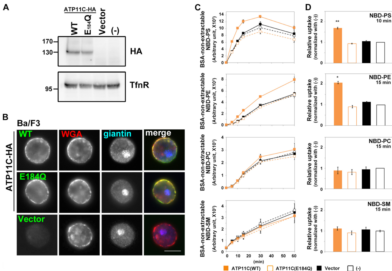
FIGURE 1. Flippase activities of ATP11C across the leaflets of the plasma membrane in Ba/F3 cells. Parental Ba/F3 cells (–) or Ba/F3 cells infected with empty retrovirus vector ( Vector ) or recombinant virus vector encoding HA-tagged ATP11C(WT) or ATP11C(E184Q) were either processed for immunoblot analysis with antibodies against HA and TfnR (as an internal control) (A) or stained with Alexa Fluor 555-conjugated wheat germ agglutinin (WGA) to visualize the plasma membrane followed by immunostaining for HA and giantin (a Golgi marker) (B). Scale bar, 10 \mu m. C, Ba/F3 cells were incubated with the indicated NBD-lipids at 15 °C for the indicated times ( x axis). After extraction with fatty acid-free BSA, the residual fluorescence intensity associated with the cells was determined by flow cytometry. Graphs are representative of two independent experiments, and results display averages from triplicates \pm S.D. D, -fold increase of NBD-lipid uptake compared with parental cells (–) is shown at the 10- (NBD-PS) or 15-min (NBD-PE, -PC, and -SM) time point from C. Graphs are representatives of three independent experiments, and results display averages from triplicates \pm S.D. (*, p < 0.0001 ; **, p < 0.0005 ). Error bars represent S.D.
