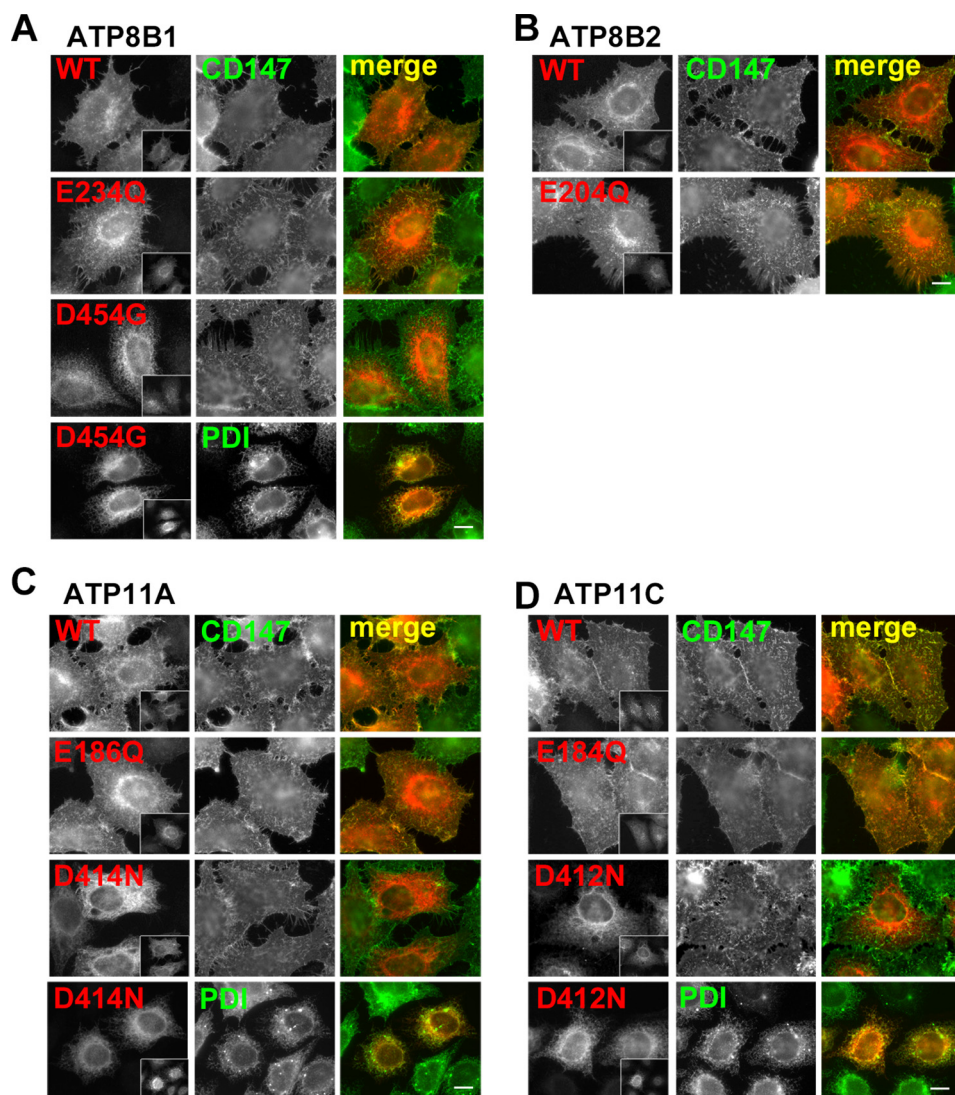
FIGURE 2. Plasma membrane localization of P4-ATPases and their ATPase-deficient mutants in HeLa cells. HeLa cells were transiently co-transfected with expression vectors for FLAG-tagged CDC50A and HA-tagged ATP8B1(WT), ATP8B1(E234Q), or ATP8B1(D454G) (a BRIC mutant, see Fig. 7) (A); ATP8B2(WT) or ATP8B2(E204Q) (B); ATP11A(WT), ATP11A(E186Q), or ATP11A(D414N) (C); or ATP11C(WT), ATP11C(E184Q), or ATP11C(D412N) (D). Before fixation, cells were incubated with Alexa Fluor 488-conjugated anti-CD147 antibody for 5 min at room temperature to label the plasma membrane. The fixed cells were then incubated with anti-HA and anti-FLAG (M2) antibodies followed by Cy3-conjugated anti-rat and DyLight649-conjugated anti-mouse secondary antibodies. For protein-disulfide isomerase (PDI; an endoplasmic reticulum marker) staining, fixed cells were incubated with anti-HA, anti-FLAG, and anti-protein-disulfide isomerase antibodies followed by Cy3-conjugated anti-rat, Alexa Fluor 647-conjugated anti-rabbit, and Alexa Fluor 488-conjugated anti-mouse secondary antibodies. Insets indicate FLAG-CDC50A-expressing cells. Scale bars , 10 \mu\text{m} .
