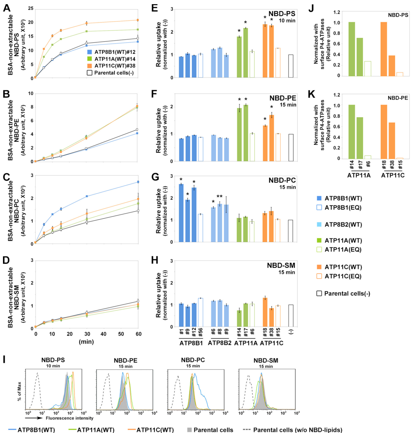
FIGURE 4. Flippase activities of P4-ATPases across the leaflets of the plasma membrane in HeLa cells. A–D, parental HeLa cells (–; open squares) and a cell line stably expressing ATP8B1 (clone 12; blue), ATP11A (clone 14; green), or ATP11C (clone 38; orange) were incubated with the indicated NBD-lipids at 15 °C for the indicated times ( x axis). After extraction with fatty acid-free BSA, the residual fluorescence intensity associated with the cells was determined by flow cytometry. Graphs are representatives of two independent experiments, and results display averages from triplicates \pm S.D. E–H, each of the clonal cell lines shown in Fig. 2 was incubated with the indicated NBD-lipids at 15 °C for 15 min (or 10 min for NBD-PS). After extraction with fatty acid-free BSA, the residual fluorescence intensity associated with the cells was determined by flow cytometry. -Fold increase of NBD-lipid uptake compared with parental HeLa cells (–) is shown. Graphs are representative of at least two independent experiments, and results display averages from triplicates \pm S.D. (*, p < 0.001 ; **, p < 0.005 ). Error bars represent S.D. I, a histogram of a representative experiment displaying the differences in the fluorescence intensity among parental HeLa cells in the absence (w/o NBD-lipids; dashed line) or presence (gray area) of NBD-lipids or a cell line stably expressing ATP8B1 (clone 12; blue), ATP11A (clone 14; green), or ATP11C (clone 38; orange) in the presence of indicated NBD-lipids at 15 °C for the indicated times. J and K, the enzymatic activities of WTs and glutamate mutants were normalized with the level of biotinylated P4-ATPases shown in Fig. 3D.
