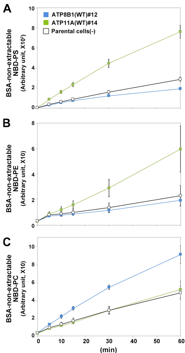
FIGURE 6. Flippase activities of P4-ATPases at 4 °C. HeLa cell lines stably expressing the HA-tagged ATP11A(clone 14) and ATP8B1(clone 12) were incubated with NBD-PS (A), NBD-PE (B), or NBD-PC (C) at 4 °C for the indicated times. The graph displays averages from two independent experiments \pm S.D. Error bars represent S.D.
