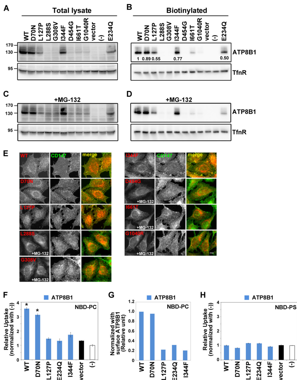
FIGURE 8. Localization and flippase activity of ATP8B1 mutants associated with cholestasis. HeLa cell lines stably expressing the HA-tagged ATP8B1 mutants indicated were established by infection of recombinant retroviral vectors. A and C , the total expression level of each ATP8B1 protein was analyzed by immunoblotting with anti-HA and anti-TfnR antibodies. 4% of the input of the biotinylation reaction was loaded in each lane. B and D , cell surface expression level of each ATP8B1 protein was analyzed after surface biotinylation. The numbers in B show the relative expression level of proteins, which were normalized with the level of the internal control, TfnR. C and D , the cells were treated with 10 \mu M MG-132 for 12 h. E , cells expressing the indicated ATP8B1 protein were processed for immunostaining. Before fixation, cells were incubated with Alexa Fluor 488-conjugated anti-CD147 antibody for 5 min at room temperature to label the plasma membrane. The fixed cells were then incubated with anti-HA antibody followed by Cy3-conjugated anti-rat secondary antibody. Cells treated with MG-132 are indicated. Scale bar, 10 \mu m. Each cell line was incubated with NBD-PC ( F ) or NBD-PS ( H ) and then processed for the flippase assay as described in the legend for Fig. 4. -Fold increase of NBD-lipid uptake compared with parental HeLa cells (-) is shown. The graph is representative of two independent experiments, and results display averages from triplicates \pm S.D. (*, p < 0.001 ). Error bars represent S.D. G , the PC flippase activities were normalized with the level of biotinylated P4-ATPases shown in B .
