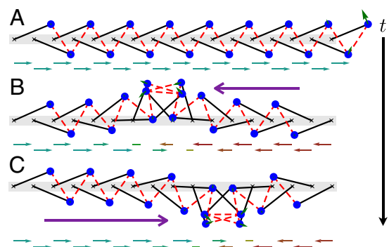
Fig. 3. The evolution of a spinner soliton arising from integrating the zero mode of a finite chain ( r/a=2 , \bar{\theta}=1.18 ), with x projections of the rotors underneath each snapshot (Movie S5). The system evolves from (A) right leaning to (B) left leaning and then back to (C) right leaning. The green arrows attached to the rotors depict the amplitude of the zero mode on each mass; note that it is always localized to the domain wall. In the spinner phase, the angle of each rotor advances by +\pi each time the soliton passes.
