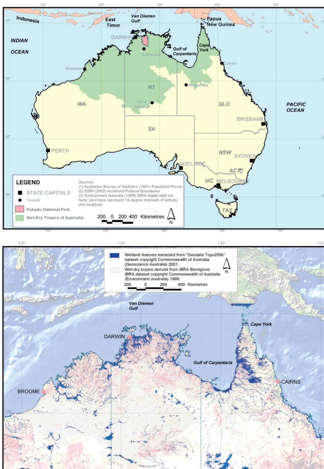
FIG. 1. The wet-dry tropics as defined on biogeographical regions (the shaded area on the upper map) with Kakadu National Park marked (Finlayson et al. , 1997a) and the distribution of wetlands (including rivers, swamps, marshes and lagoons/ponds) (from Lowry and Finlayson, 2004).
