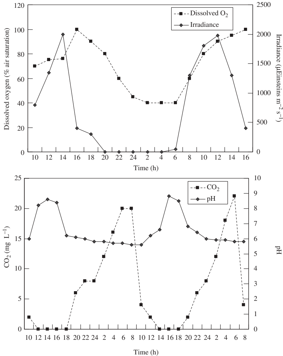
FIG. 6. Daily changes in water quality in mixed stands of emergent herbs and grasses on the Magela floodplain during the wet season (from B. Bailey, unpubl. res. 1995). (Dissolved oxygen units, percentage air saturation; irradiance, \mu\text{Einsteins m}^{-2} \text{s}^{-1} ; carbon dioxide, \text{mg L}^{-1} ).
