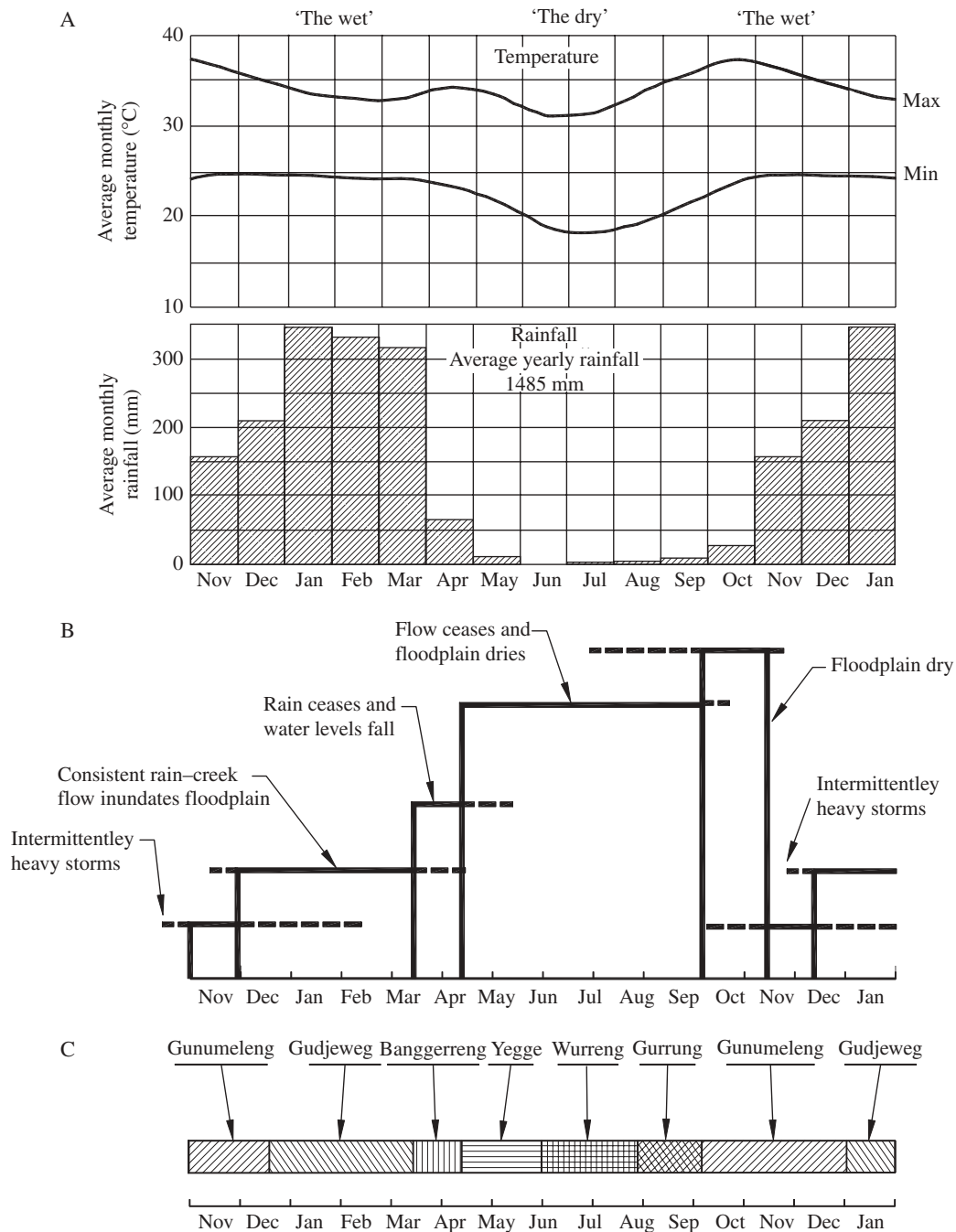
FIG. 2. Generalized representation of: (A) the climate in Darwin in the Australian wet–dry tropics; (B) hydrological changes on the Magela floodplain in Kakadu National Park (variability is represented by dashed lines); and (C) an Aboriginal calendar from Kakadu National Park. A 14 month period is shown to illustrate the extension of seasons across the calendar year. The meteorological information was derived from Hoatson et al. (2000), hydrological information was adapted from Sanderson et al. (1983) by Finlayson et al. (1990a), and the aboriginal calendar from Ovington (1986) and Morris (1996). The aboriginal seasons are described in the following manner: Gunumeleng, pre-monsoon season; Gudjeweg, monsoon season; Banggerreng, harvest time; Yegge, cool weather time; Wurreng, early dry season; Gurrung, hot dry season.
