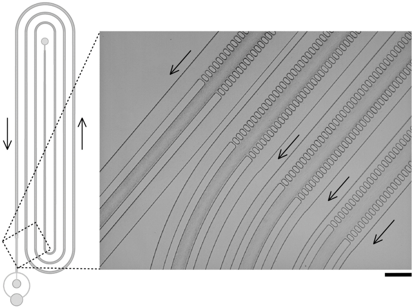
Figure 6. CIF-based device for enrichment of platelets in platelet-rich plasma (PRP). Overall design of the device is shown schematically on the left. The value of f_{gap} for this device was 1.04 \times 10^{-4} . A close-up view of a representative functional device in operation, showing incremental concentration of platelets in successive legs of the CIF array, is shown on the right. The depth of the device was 150 \mu\text{m} \pm 5 \mu\text{m} ; the width of the central channel was 125 \mu\text{m} and the final width of the side channels was 140 \mu\text{m} such that the ratio of total flow into the side channel collection port was \sim 2.5 \times that into the central collection port. The device consistently retained >80\% of platelets in the central channel, representing a \sim 3 \times enrichment in platelet concentration overall. Arrows indicate direction of flow. Scale bar is 250 \mu\text{m} .
