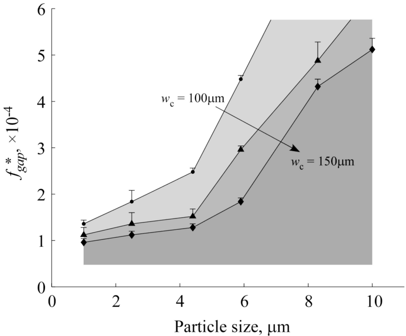
Figure 3. Effect of central channel width ( w_c = 100\mu\text{m} , 125\mu\text{m} , 150\mu\text{m} ) on the threshold value of the filtration fraction per gap, f_{gap}^* , observed for particles of different size.
