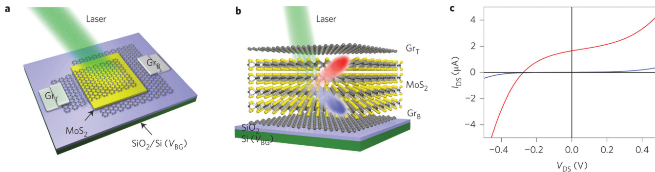
Figure 1. Photocurrent generation in vertical heterostructures of graphene–MoS 2 –graphene a , Schematic illustration of the three-dimensional device layout. b , Schematic illustration of the side view of the device, with the semiconducting multilayer MoS 2 sandwiched between the Gr T and Gr B electrodes. Red and blue colours indicate electrons and holes, respectively. The silicon substrate can be used as a back-gate electrode with 300 nm SiO 2 as the dielectric layer. c , Experimental current–voltage characteristic of the vertical device in the dark (blue) and under illumination (red) by a focused laser beam (wavelength, 514 nm; power, 80 μW; spot size, 1 μm).
