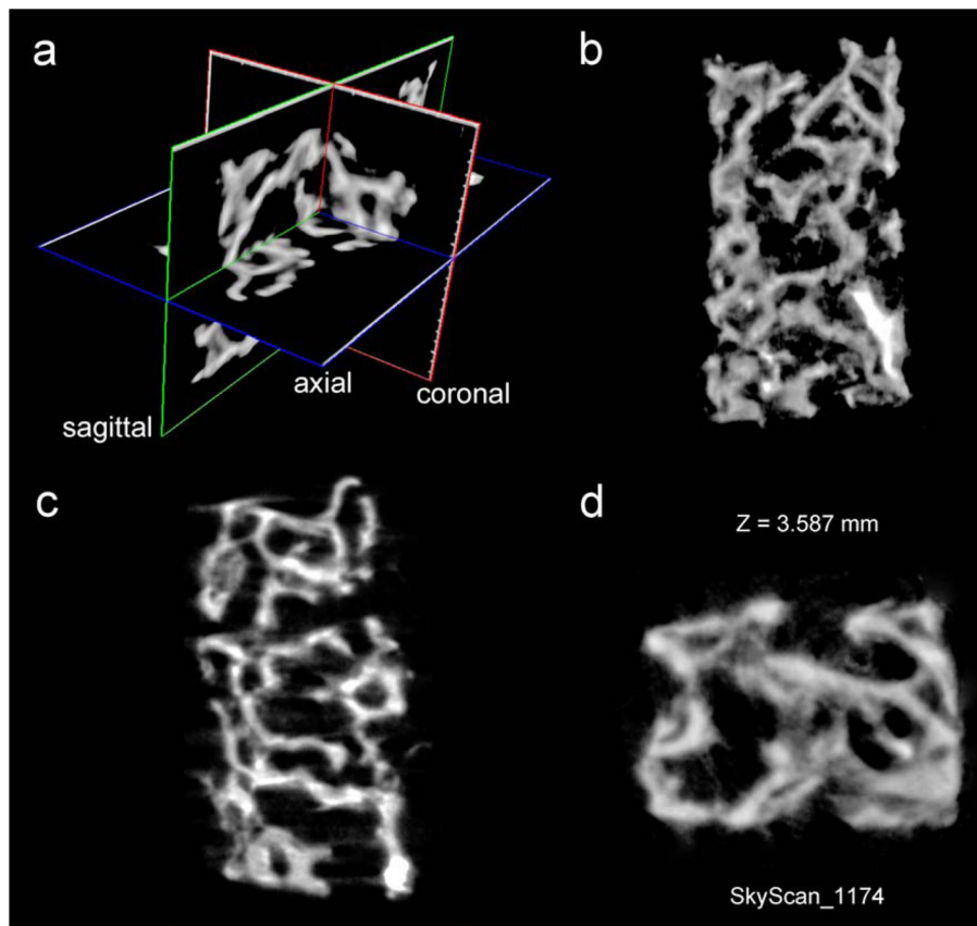
Figure 5. Micro-computed tomography of a piece of delipidated and demineralized porcine trabecular bone that has been infiltrated with acac-inhibited YSZ precursors
