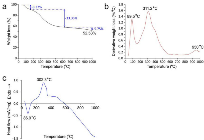
Figure 4. Thermal analyses of YSZ-infiltrated collagen scaffolds
