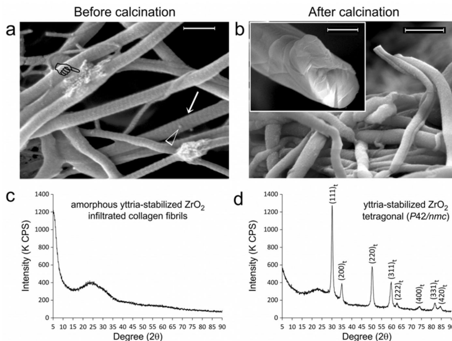
Figure 1. Infiltration of yttrium-stabilized zirconia (YSZ) into reconstituted type I collagen scaffolds
