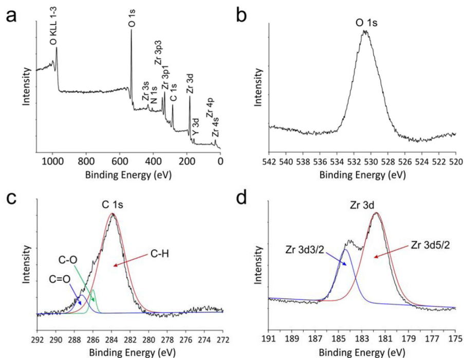
Figure 3. X-ray photoelectron spectroscopy (XPS) characterization of YSZ-infiltrated collagen scaffold
