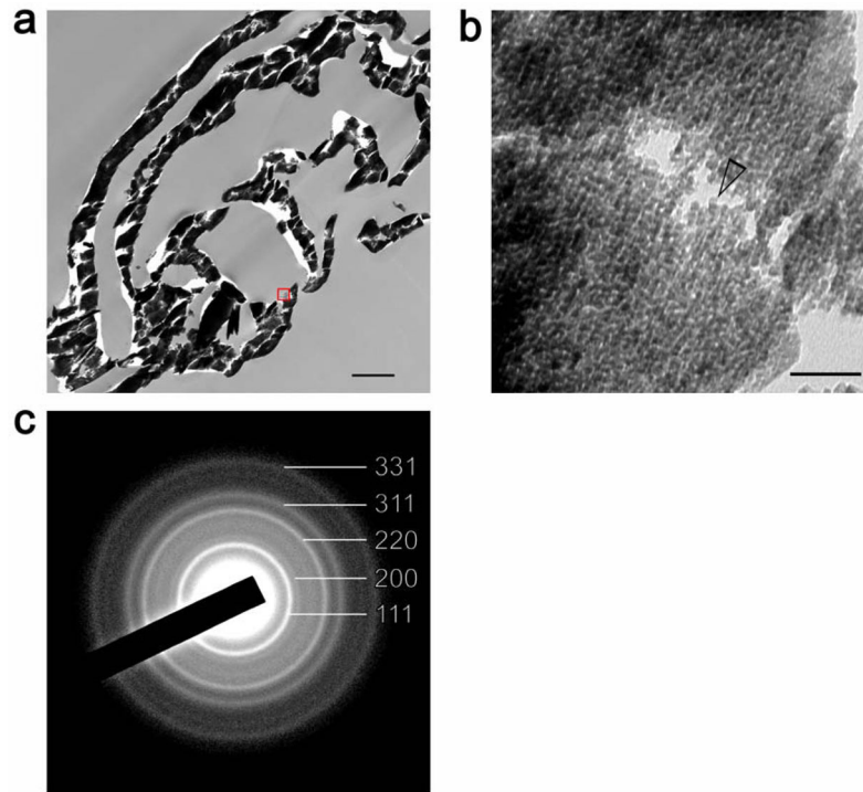
Figure 6. YSZ-infiltrated collagen scaffold that has been sintered in atmospheric air to 1,000°C a) low magnification image of a part of the organic matter-free, highly electron-dense YSZ scaffold. Bar = 1 μm. b) High magnification image taken from a leaflet of the sintered mineralized scaffold (red box in previous image) showing the presence of YSZ nanoparticles ( \approx 5 nm in diameter – open arrowhead). Bar = 50 nm. c) Selected area electron diffraction showing ring patterns characteristic of the tetragonal structure of the sintered polycrystalline YSZ nanoparticles.
