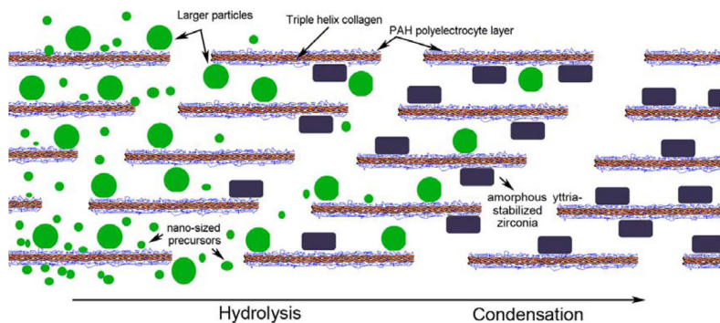
Figure 7. Schematic of the process of intrafibrillar deposition of yttria-stabilized zirconia (YSZ) within a collagen fibril
