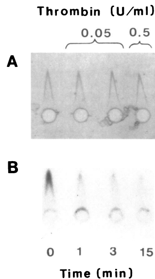
Figure 6. Immunoelectrophoresis of thrombin-treated V_0 VIII:CAg incubated with ^{125}\text{I} -Fab, and electrophoresed against rabbit anti-human VIII:RAG. At the indicated times after thrombin addition (0.05 U/ml final concentration), proteolysis was stopped with ^{125}\text{I} -Fab-inhibitor-PEG solution. The last sample was incubated for 15 min with 0.5 U/ml thrombin. Coomassie Blue-stained precipitin arcs (A) were autoradiographed (B).
