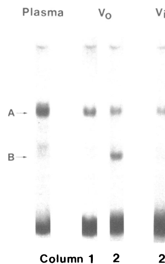
Figure 4. Autoradiographs of ^{125}I -Fab-treated plasma, V_0 , and V_i gel filtration fractions analyzed by SDS-3% PAAGE. Apparent molecular weights of the major free VIII:CAG species, calculated from migration distances of ^{125}I -Fab-antigen complexes on SDS-4% PAAGE, are A, 2.4 \times 10^5 , and B, 1 \times 10^5 . Aliquots of a single plasma sample were gel filtered on columns, equilibrated (column 1) or not (column 2) with freshly prepared inhibitor-containing buffer. V_0 VIII:CAG (column 1) and V_i VIII:CAG (column 2) had the same molecular weight, but V_0 VIII:CAG of column 2 was degraded.
