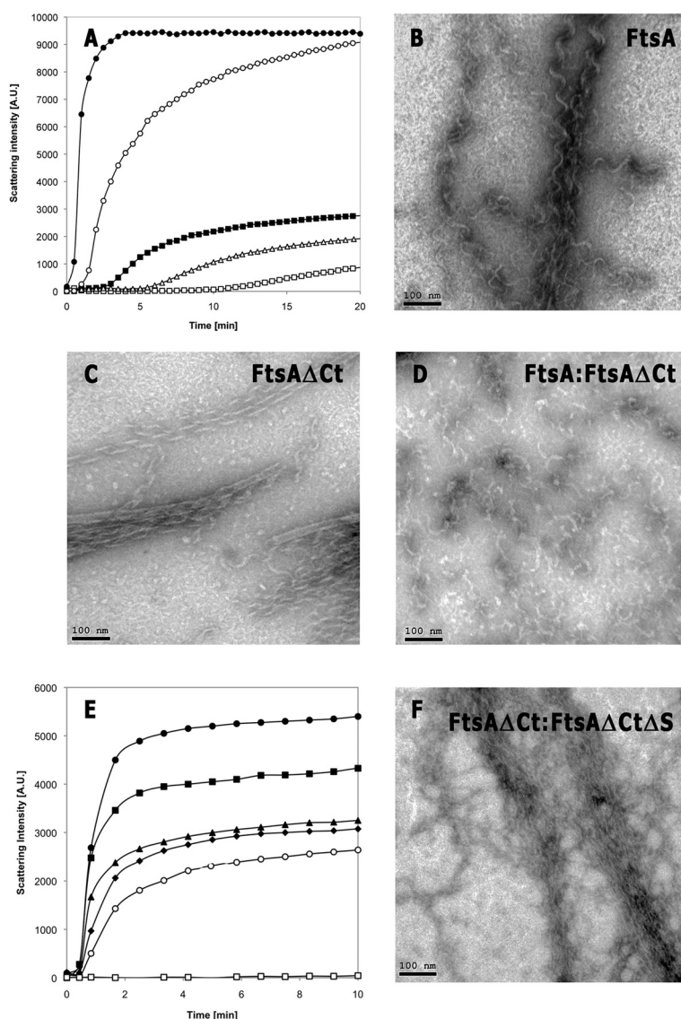
FIG 1 In vitro polymerization of FtsA proteins. (A) Light-scattering measurements of 5 \mu\text{M} FtsA + (○), 5 \mu\text{M} FtsAΔCt (●), 2.5 \mu\text{M} FtsA + (□), 2.5 \mu\text{M} FtsAΔCt (■), and a mixture of 2.5 \mu\text{M} FtsA + with 2.5 \mu\text{M} FtsAΔCt (△) after the addition of 2 mM ATP. A.U., arbitrary units. (B to D) Electron microscopy of polymers formed by 5 \mu\text{M} FtsA + (B), 5 \mu\text{M} FtsAΔCt (C), and a mixture of 2.5 \mu\text{M} FtsA + and 2.5 \mu\text{M} FtsAΔCt (D). Bars, 100 nm. (E) Light-scattering measurements of 5 \mu\text{M} FtsAΔCt (●), 5 \mu\text{M} FtsAΔCtΔS (□), or 5 \mu\text{M} FtsAΔCt in the presence of 1.25, 2.5, 3.75, and 5 \mu\text{M} FtsAΔCtΔS (■, ▲, ◆, and ○, respectively). (F) Electron microscopy images of polymers formed by a mixture of 5 \mu\text{M} FtsAΔCt and 2.5 \mu\text{M} FtsAΔCtΔS. Bar, 100 nm.
