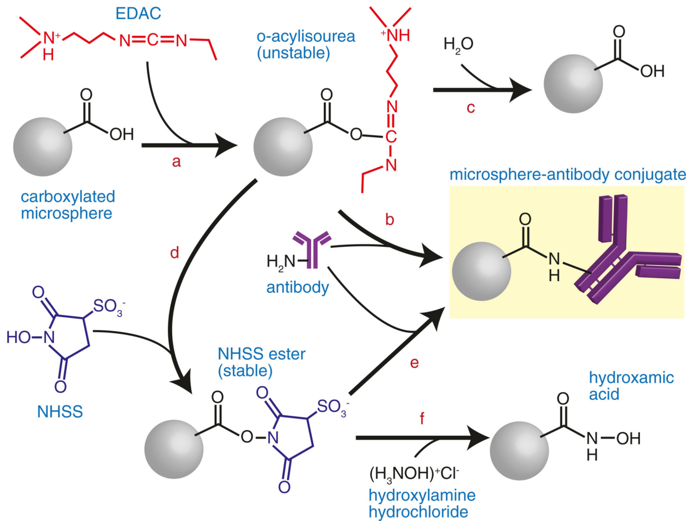
Fig. 6. Coupling antibodies to optical trapping microspheres. First, a microsphere bearing surface carboxyl groups reacts (a) with the carbodiimide EDAC (1-ethyl-3-(3-dimethylaminopropyl)carbodiimide) to form an unstable O -acylisourea intermediate. This short-lived species is reactive toward primary amines and thus capable of forming stable, covalent amide bonds with lysyl residues on the antibody surface (b) and yielding an isourea byproduct (not shown). However, this O -acylisourea is also readily and rapidly hydrolyzed, yielding the original carboxyl group (c). Adding NHSS (3-sulfo- N -hydroxysulfosuccinimide) to the reaction greatly enhances microsphere–antibody coupling efficiency by forming a relatively water-stable, but amine-reactive NHSS ester (d) that can likewise bind antibodies (e). BSA (not shown) is added with the antibody and also binds via its surface lysines, thus blocking the remainder of the microsphere surface. After antibodies and BSA are bound, any residual NHSS esters are removed by adding hydroxylamine (f), which reacts with the ester to form hydroxamic acid
