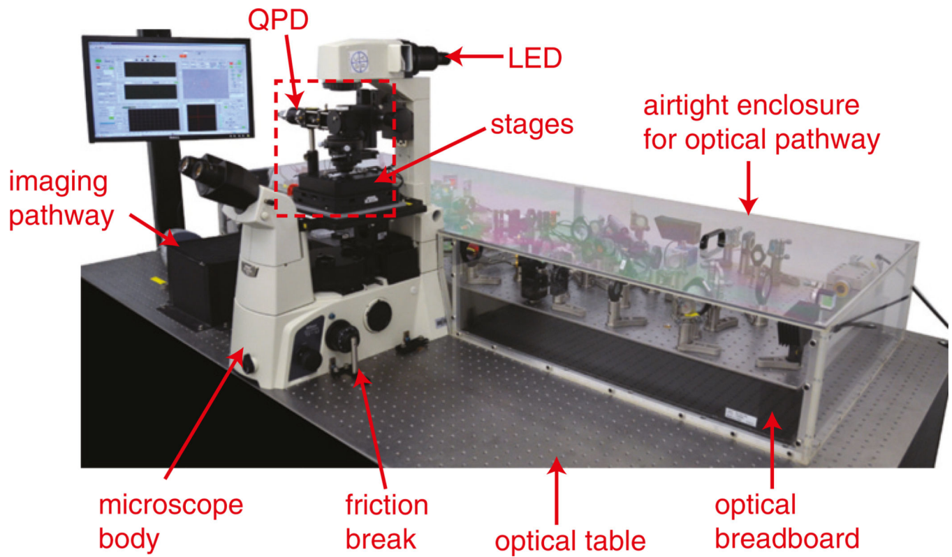
Fig. 4. Force-fluorescence trapping microscope. Note the optical pathway elevated on an optical breadboard and enclosed in an airtight box. The friction break [165] consists of an optical post or other rigid element bolted firmly to the table and pressed against the microscope fine-focus knob to prevent drift of the objective over time. The region demarcated by the red dashed line (back focal plane imaging arm) is shown in greater detail in Fig. 12. Refer also to Fig. 3
