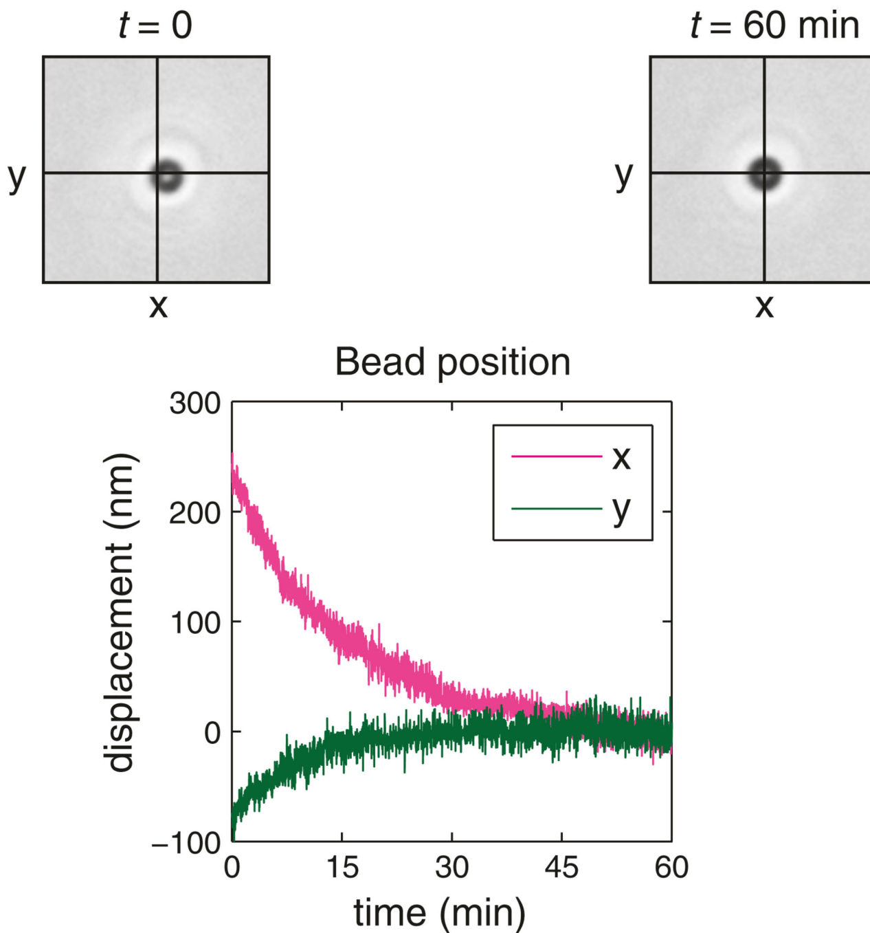
Fig. 8. Thermal equilibration of the optical tweezers laser pathway. When the optical trapping laser is initially powered on, the trap center is typically offset from its previous stable position ( left-hand image ; the cross to the upper left of the bead is the stable position to which the bead moves after the optical elements in the pathway expand due to heating by the trapping laser). The new position is typically very close (tens of nanometers) to the stable position during the preceding use of the instrument ( right-hand image ). The graph shows a representative example of microsphere movement over time as the optical pathway
