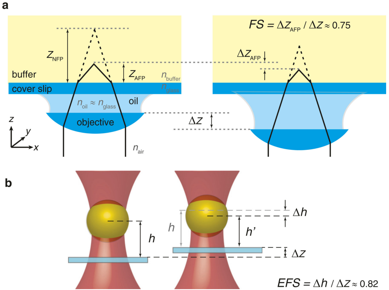
Fig. 16. The focal shift and its effects on bead–cover slip separation. (a) Ray diagram for a collimated beam focused by an oil immersion microscope objective. Although the indices of refraction are closely matched between the objective, immersion oil, and cover slip ( n_{\text{oil}} \approx n_{\text{glass}} \approx 1.51 ), the refractive index of the sample buffer is significantly smaller ( n_{\text{buffer}} \approx n_{\text{water}} = 1.33 ). This causes the rays to refract at the interface, bringing the actual focus position ( Z_{\text{AFP}} , measured relative to the cover slip surface) closer to the objective than the nominal focus position ( Z_{\text{NFP}} ) expected if the refractive indices were equal (dashed rays). Z_{\text{AFP}} depends on the indices of refraction and on the distance the beam travels in each medium (glass/oil vs. buffer), which is determined by the separation between the cover slip and objective. A change \Delta Z in this separation (due to movement of the objective or cover slip) induces a corresponding change \Delta Z_{\text{AFP}} in the actual focus position, which is linear with \Delta Z over several micrometers. The proportionality constant relating \Delta Z_{\text{AFP}} to \Delta Z is referred to as the focal shift, FS (which is defined differently by some authors, as the difference [Z_{\text{NFP}} - Z_{\text{AFP}}] ). Using high-NA oil-immersion objectives and aqueous buffer, a full electromagnetic treatment of the problem gives FS \approx 0.75 . (b) In optical tweezers, the figure of interest is not the focal shift per se, but rather the effective focal shift ( EFS ), defined
