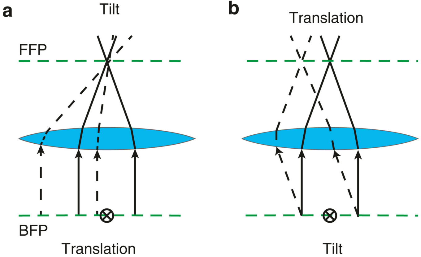
Fig. 9. Important optical relationships for focusing a collimated beam. BFP, back focal plane; FFP, front focal plane. Solid rays represent a beam perfectly aligned with and centered on the optical axis. (a) Pure translation of the beam in the back aperture leads to tilting of the beam as it focuses in the FFP, but does not change the position of the focus. This induces asymmetry in intensity pattern of the retroreflected beam. (b) Pure tilting of the beam in the BFP leads to translation of the focus in the FFP, essentially without affecting the beam angle as it approaches the FFP. This shifts the position of the intensity pattern of the retroreflected beam, with minimal effects on the intensity distribution
