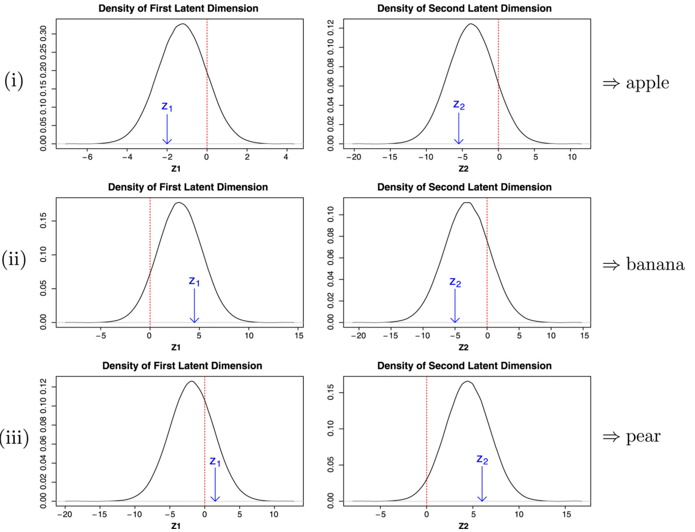
Fig. 8. Latent variable formulation of nominal responses.
