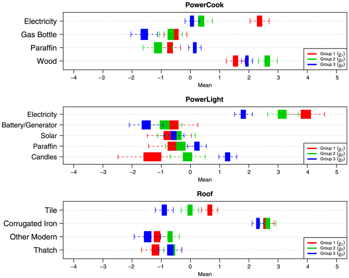
Fig. 4. Box plots of MCMC samples of the dimensions of the cluster means, \mu_g , corresponding to nominal items. The first plot shows box plots of the means of the latent dimensions relating to the PowerCook item, the second shows the means of the dimensions representing the PowerLight item and the third shows the means of the dimensions corresponding to the Roof item.
