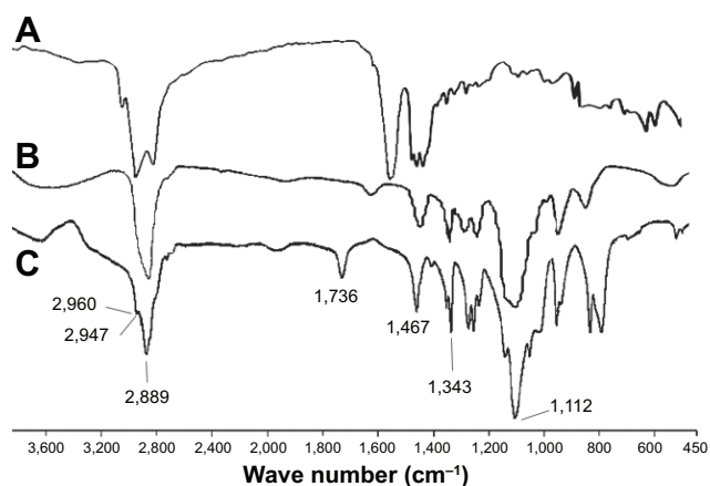
Figure 1 Fourier transform infrared spectra of mPEG-OA nanocarriers.
