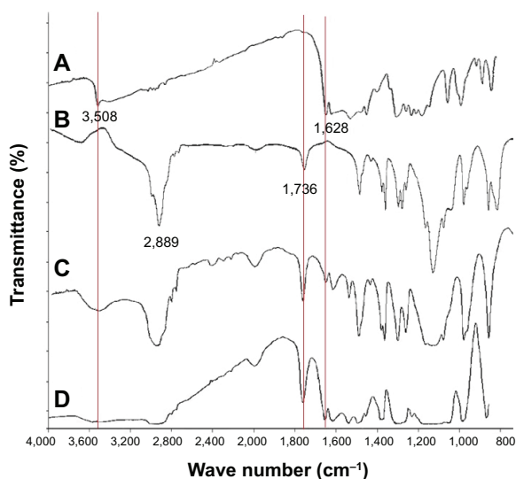
Figure 4 Fourier transform infrared spectra of curcumin, void mPEG-OA nanocarriers, curcumin encapsulated in mPEG-OA nanocarrier, and a physical mixture of curcumin with void mPEG-OA nanocarriers.
