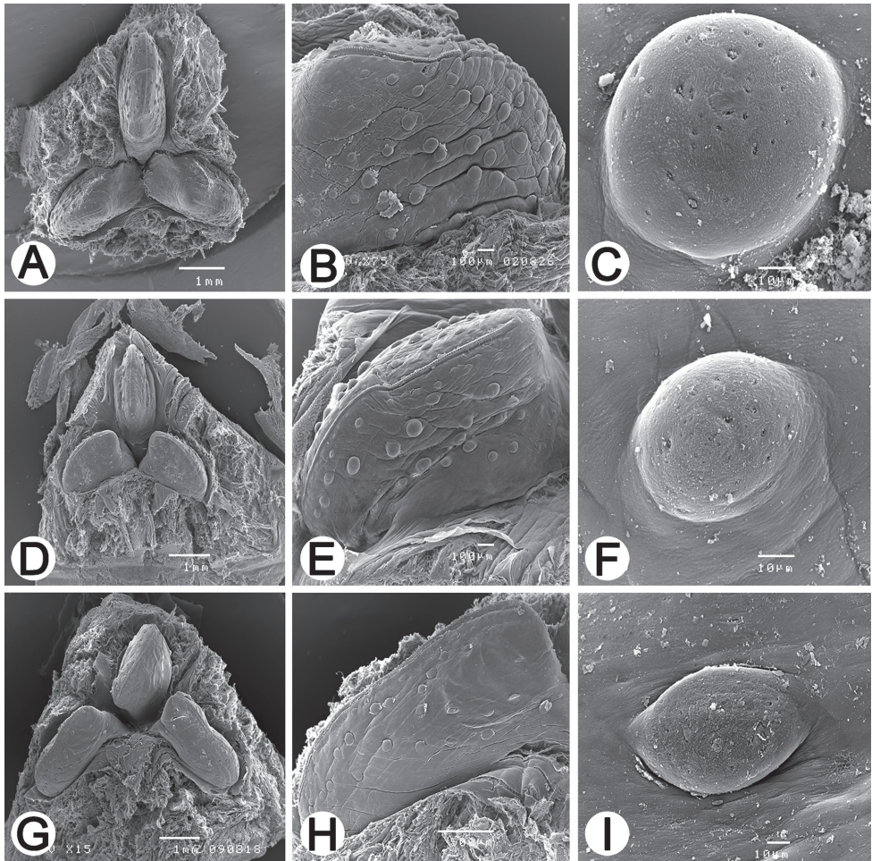
Figure 5. SEM images of the jaws of A–C Hirudinaria javanica CUMZ 3404 from Nakhon Phanom D–F Hirudinaria manillensis CUMZ 3403 from Nakhon Phanom, and G–I Hirudinaria sp. CUMZ 3405 from Nakhon Phanom. ( A, D, G ) overall jaw, ( B, E, H ) each jaw characteristic, and ( C, F, I ) salivary papillae.
