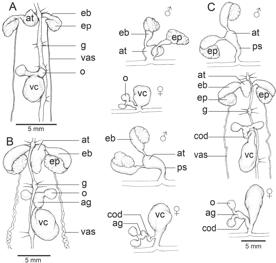
Figure 4. Illustrations of the reproductive system of A Hirudinaria javanica CUMZ 3404 from Nakhon Phanom, B Hirudinaria manillensis CUMZ 3403 from Nakhon Phanom, and C Hirudinaria sp. CUMZ 3405 from Nakhon Phanom. Abbreviations are: ag = albumin gland, at = atrium, cod = common oviduct, eb = ejaculatory bulb, ep = epididymis, g = ganglion, o = ovary, ps = penis sheath, vas = vas deferens, vc = vagina duct.
