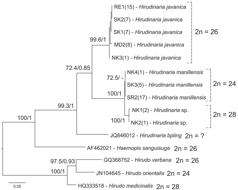
Figure 8. Phylogenetic relationships of the genus Hirudinaria and their related species, with chromosome number data. Tree topology was obtained from ML analysis based on a 658 bp fragment of the mitochondrial COI gene (DNA barcode region). Nodes with a 0.95 or higher bipartition posterior probability for BI and/or 70% or higher bootstrap value for ML were regarded as sufficiently resolved nodes, and are shown for the major clades (ML/BI). Numbers in parentheses refer to sampling localities in Figure 1 and the list in Table 1. Chromosome data of the related species were taken from Vitturi et al. (2002) and Utevsky et al. (2009).
