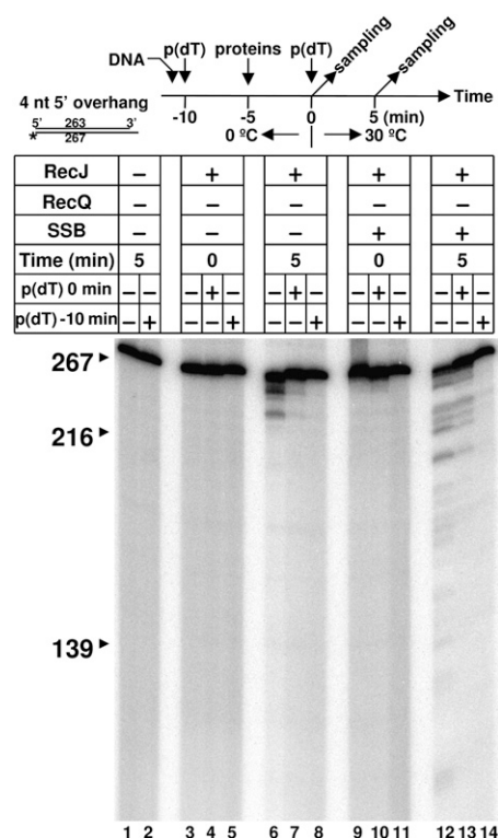
Fig. 3. Resection of dsDNA by RecJ nuclease is processive. Resection performed in the presence of scavenger DNA, poly(dT) (40- \mu M nucleotides). 32 P-labeled HindIII-cut dsDNA was used as described in Materials and Methods . After incubation for the time indicated (0 or 5 min), samples were analyzed by PAGE. Reactions without scavenger DNA are lanes 1, 3, 6, 9, and 12. In the reactions of lanes 4, 7, 10, and 13, scavenger DNA were added at 0 min. To show that the scavenger is effective, poly(dT) was added 5 min before mixing dsDNA with RecJ [shown as “p(dT) -10 min”: lanes 2, 5, 8, 11, and 14]. The reaction scheme is summarized at the top.
