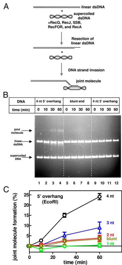
Fig. 1. RecA/RecFORQJ-mediated joint molecule formation is sensitive to the end structure of the linear dsDNA to be resected. (A) Schematic of RecA/RecFORQJ-mediated joint molecule formation between linear dsDNA and supercoiled dsDNA (28). The reaction comprises two concerted steps. In the first step, RecJ—with the help of RecQ and SSB—processes the linear dsDNA. In the second step, the RecFOR proteins load RecA onto the processed linear DNA, which is followed by RecA-promoted joint molecule formation. (B) Joint molecule formation using linear dsDNA with 4-nt 5'-overhangs (lanes 1–4), blunt-ends (lanes 5–8), or 4-nt 3'-overhangs (lanes 9–12). EcoRI, SmaI, and PstI were used to generate the linear dsDNA. Samples were analyzed by agarose gel electrophoresis followed by ethidium bromide staining. (C) Effect of linear DNA-end structure on joint molecule formation was investigated using EcoRI-cut pUC19 DNA that was filled-in to produce the overhangs indicated. Joint molecule assays, such as those shown in B, were quantified to determine the percentage of the limiting linear dsDNA that was converted into joint molecules. Each experiment was performed twice; the error bars show standard error (SE), unless smaller than the symbol.
