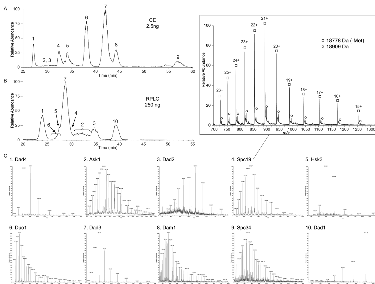
Figure 1. (A) Electropherogram of Dam1 complex subunit separation by sheathless CESI-MS (2.5 ng loaded). CE separation conditions: PEI coated capillary; voltage -30 kV; BGE 5% acetic acid, 5% IPA. (B) Chromatogram of Dam1 complex subunit separation by RPLC-MS (250 ng loaded). RPLC separation conditions: 75 \mu\text{m} i.d. capillary with 5 \mu\text{m} 1000 \text{\AA} PSDVB resin; flow rate of 300 nL/min. For more details see Methods and Materials section. (C) Representative MS precursor scans of the 10 protein subunits from Dam1 complex. Subunits 1–9 are from (A) the CESI-MS experiment; subunit 10 is from (B) the RPLC-MS experiment. The insert is the zoomed-in spectrum for Spc19p, showing two different protein envelopes that represent the sequence predicted form (indicated by \circ , 18 909 Da, average mass) and the N-terminal methionine excision form (indicated by \square , 18 778 Da, average mass).
