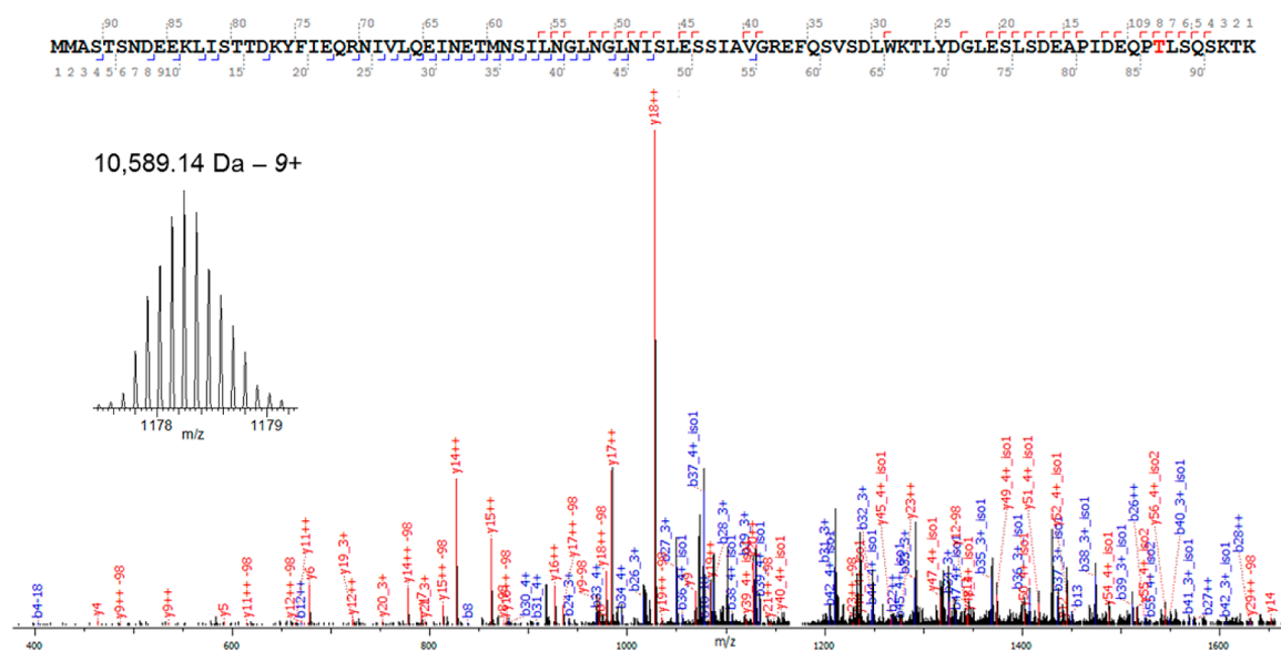
Figure 4. CID fragmentation of selected precursor ion ( 1178.13^{9+} ) and protein identification along with the fragmentation map for Dad1p (measured MW = 10 589.14 Da). The MS/MS spectrum corresponded to the identification of Dad1p with one phosphorylation site (T87, in red) localized. The b - and y -ions were indicated as blue and red in the fragmentation map and the MS/MS spectrum.
