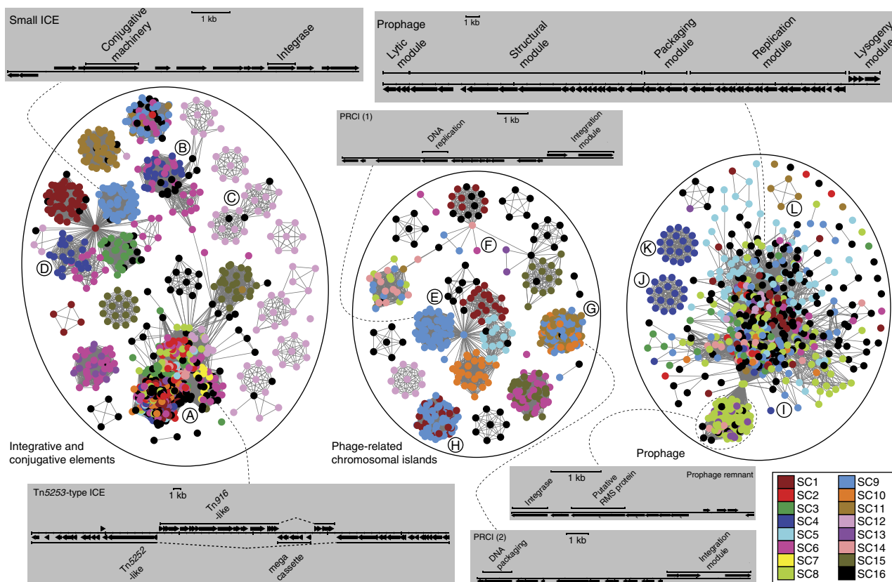
Figure 3 | Mobile genetic elements found in the pneumococcal population. The 2,226 MGE sequences identified in the collection that could be classified as derived from a putative ICE, PRCI or prophage are each represented by a node, coloured according to the sequence cluster of the host in which it was found as displayed in the key. These are linked by vertices based on their similarity in terms of COGs using the Mountford index and classified using functional domains that appear characteristic of different MGE types. Clusters of nodes described in the text are annotated with letters. The grey boxes display the annotation of representative nodes, indicated by the dashed lines, from the main clusters in the network.
