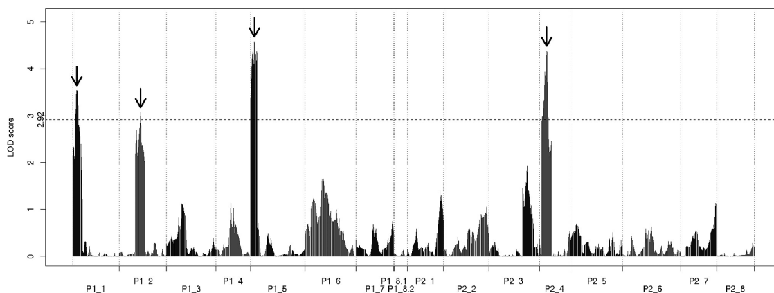
Fig. 5. Logarithm of the odds (LOD) score profile of the quantitative trait loci analysis of main stem length. Map positions are shown on the x-axis. The horizontal dashed line shows the 5% threshold of LOD score (2.92) obtained from a permutation test. Arrows show the detected peaks of LOD scores.
