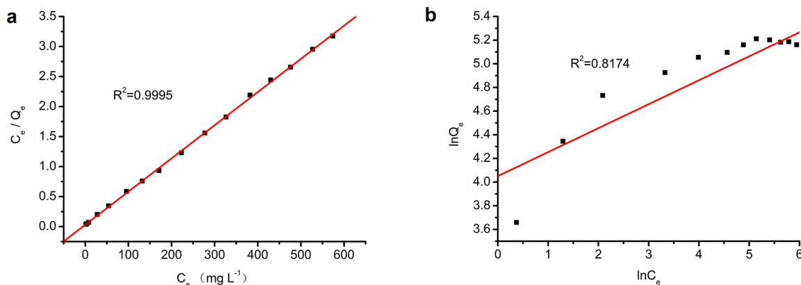
Figure 11. Plots of Langmuir (a) and Freundlich (b) isotherms. doi:10.1371/journal.pone.0108647.g0011
