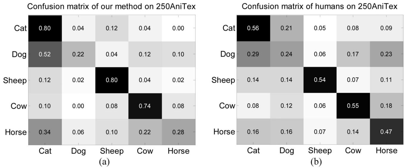
Fig. 6. The confusion matrices for (a) our algorithm and (b) humans on the 250AniTex dataset.
