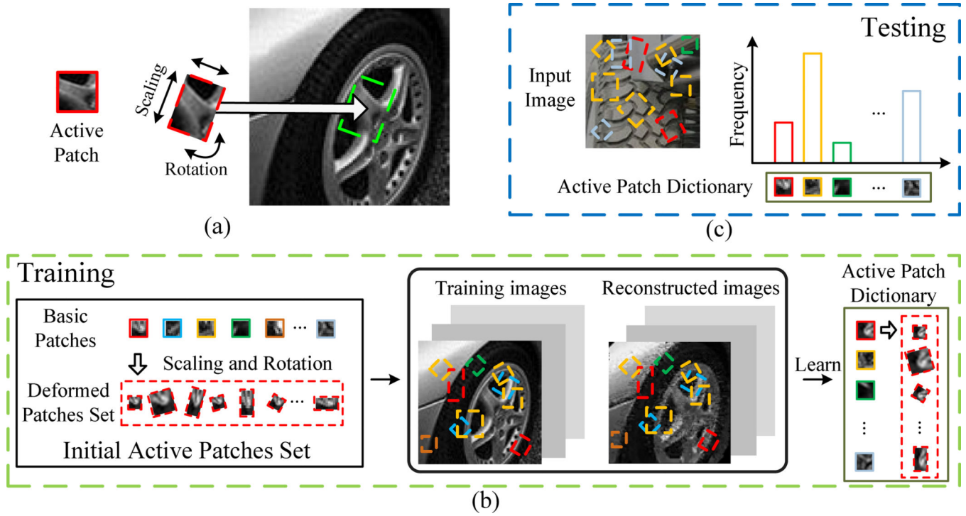
Fig. 2. Illustration of our approach. (a). An active patch will take actions to best fit the image region near a target position (the green rectangle region in the image) in the best way. The actions consist of the combination of scaling and rotation. (b). To implement these actions efficiently, each active patch consists of a basic patch (e.g. the patch in the solid red rectangle in the left panel of (b)) and a deformed patches set (e.g. the patches in the dashed red rectangle). Given an image position, the active patch will find one of its deformed patches that has the maximum matching score with the image region near this position. If the score is larger than a threshold, the active patch is “fired” at the image region. In this way, the images can be reconstructed and represented by a set of firing active patches. We learn the active patch dictionary in a greedy manner using criteria based on the reconstruction of the training images. (c). The histogram of firing frequencies of the active patches in the dictionary will be treated as the feature for appearance classification. (Best viewed in color)
