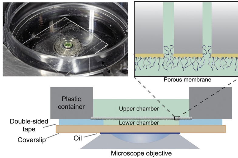
FIGURE 17.1. Device setup. Photograph (top left), porous membrane diagram (top right), and schematic representation (bottom) of biomimetic NPC device.
