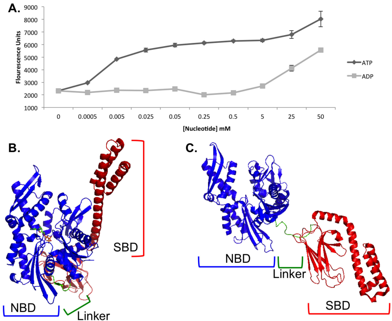
Figure 1. Recombinant GFP-Hsp70i is readily captured on \gamma -phosphate linked ATP resin and is competitively released with ATP/ADP, consistent with nucleotide induced conformational changes
