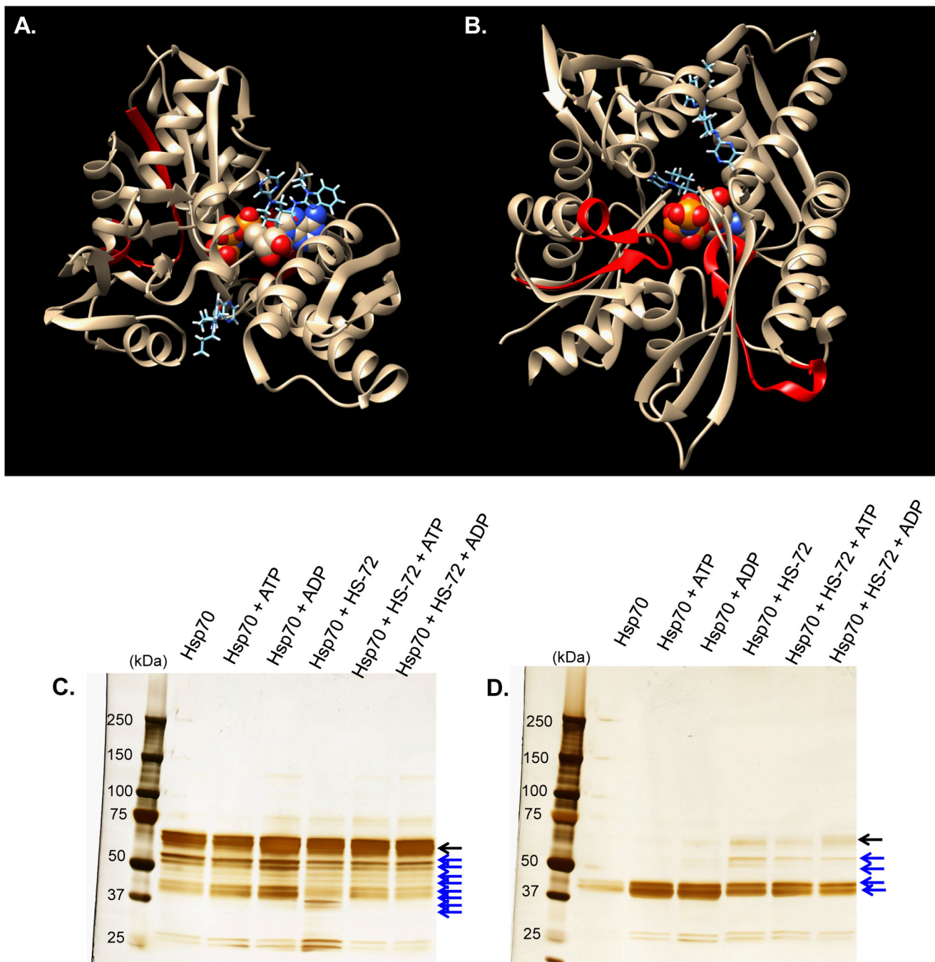
Figure 5. Molecular modeling and native protein digestion studies supports HS-72 as an allosteric inhibitor of Hsp70i
