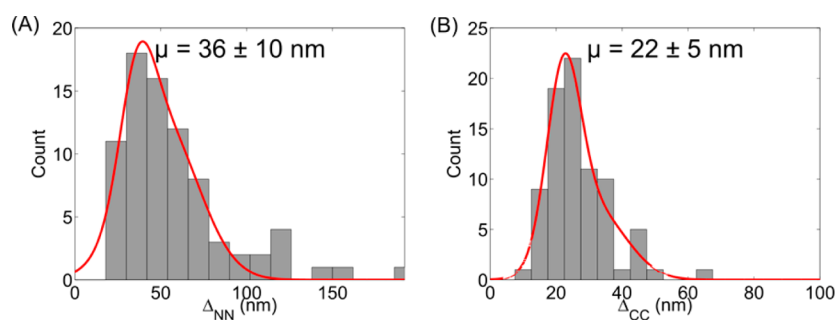
Figure 4. Distributions of (A) the distances between N-terminus of subunits of human Piezo1 ( \Delta_{NN} ) and (B) the distance between C-terminus ( \Delta_{CC} ). Fitting curves f(x) = A_1 \exp[-(x - \mu)^2 / (2\sigma_1^2)] + A_2 \exp[-(x - \sqrt{2}\mu)^2 / (2\sigma_2^2)] give (A) \mu = 36 \pm 10 nm (Mean \pm SD) for \Delta_{NN} and (B) \mu = 22 \pm 5 nm (Mean \pm SD) for \Delta_{CC} .
