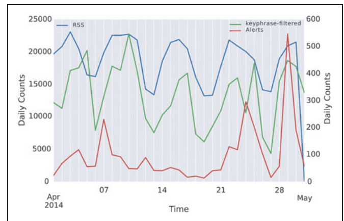
FIG. 5. Data reduction from Really Simple Syndication (RSS) feeds to alerts in an EMBERS civil unrest forecasting model.
