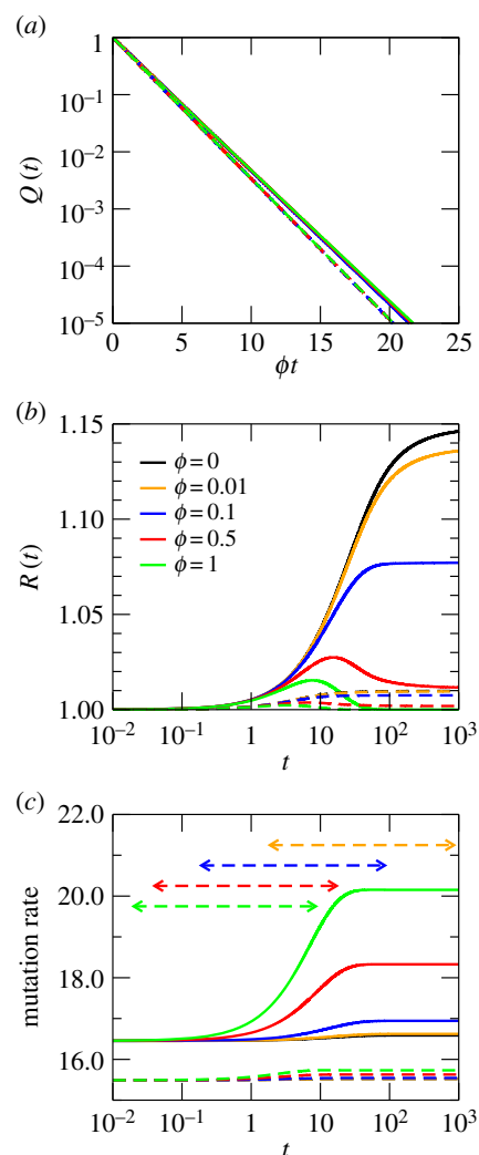
Figure 4. Dynamics of a RW on two different RNA secondary structure NNs with z = 36 . Sizes are M = 1965 (dashed lines) and M = 21\,908 (solid lines). (a) Probability Q(t) that the RW stays on the network after a time t . (b) Overdispersion of the network. (c) Mutation rate. Times t_{19\%}(\phi) and t_{99\%}(\phi) are only shown for the largest network. The assortativity is r > 0.90 . For the sake of comparison, these plots share scale with figure 1.
