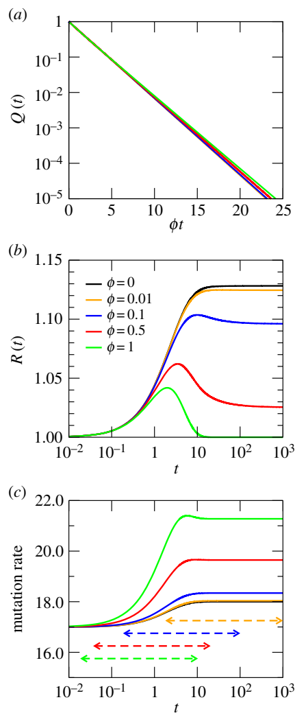
Figure 1. Dynamics of RWs on an Erdős–Renyi random network with M = 20\,000 nodes and average degree \langle k \rangle = 18 . (a) Probability Q(t) that the RW stays on the network after a time t . (b) Overdispersion of the network. (c) Mutation rate or acceleration of the molecular clock. The time interval through which the number of trajectories remaining on the network decreases from 99% to 1% is represented as a horizontal dashed line limited by two arrows, with the same colour as the \phi curve they correspond to. The same code is used in subsequent corresponding panels for other networks. The measured assortativity for this finite network is r \simeq 0.018 .
