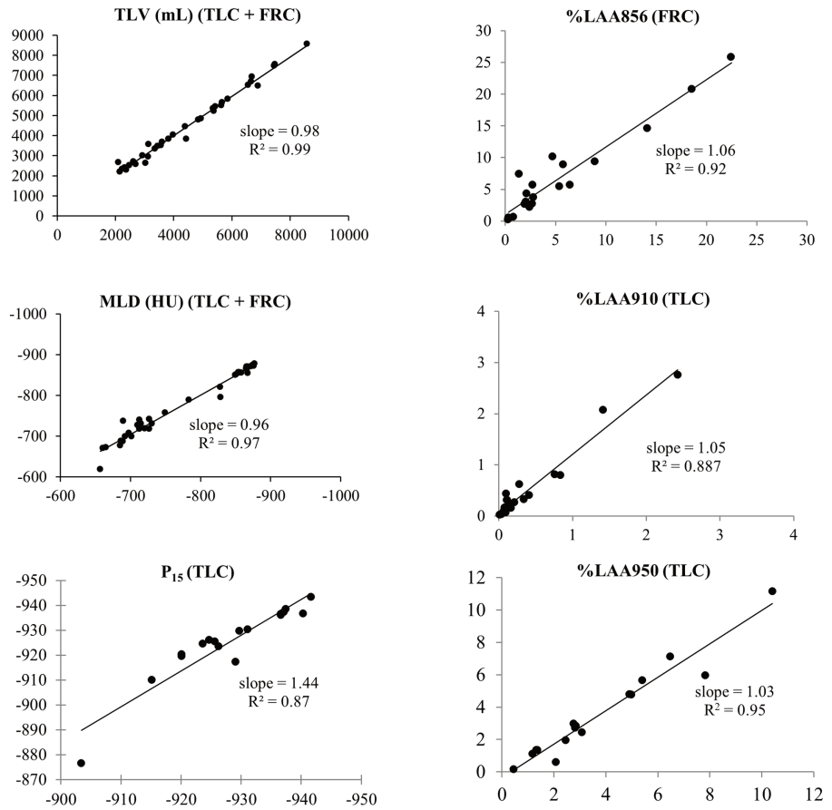
Figure 1: Linear regression plots for five whole lung density-based metrics plus total lung volume (TLV). LAA metrics are percentages in the horizontal and vertical axes.
