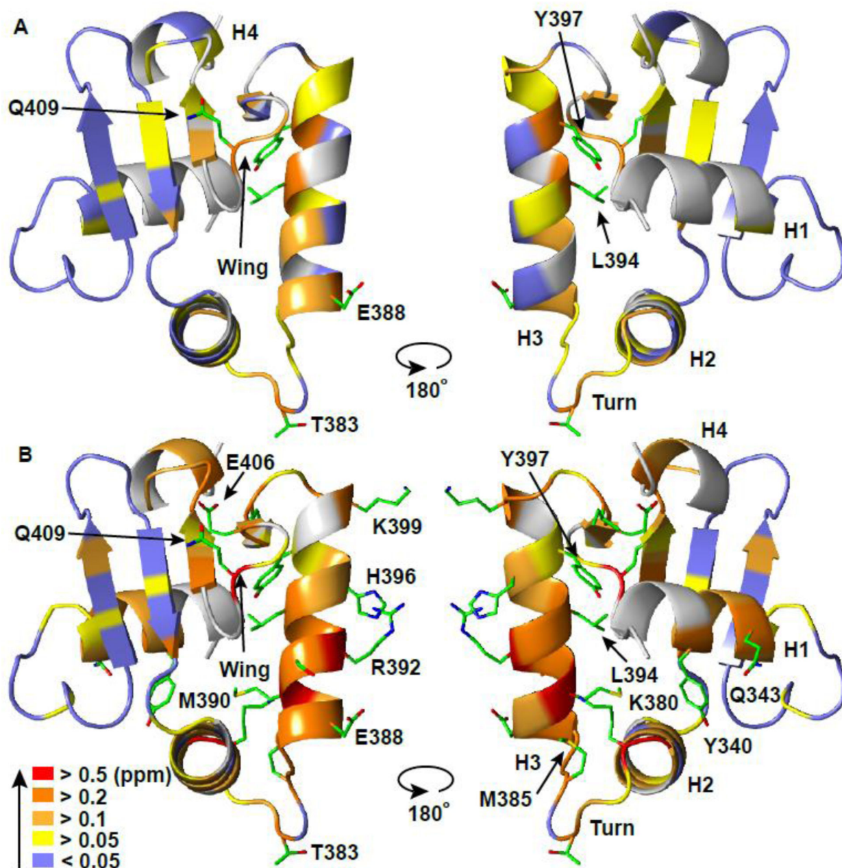
Fig. 5. ETV6 ETS domain binds specific and non-specific DNA via the same canonical interface. The amide chemical shift perturbations (CSP's, \delta = \{(\delta_H^2 + (0.154 \delta_N)^2)^{1/2}\} ) for (A) ETV6 D446 -DNA nonsp and (B) ETV6 D446 -DNA sp with respect to unbound ETV6 R426 are mapped onto the crystal structure of ETV6 R426 -DNA sp-cryst (DNA not shown). Residues (backbone cartoon) are color-coded in the indicated CSP ranges. Prolines and unassigned residues are in grey. Side chains are shown for residues in (A) with CSP > 0.2 ppm and in (B) with CSP > 0.4 ppm. See Figure 1 and Supplemental Figures S1 and S4 for the original data.
