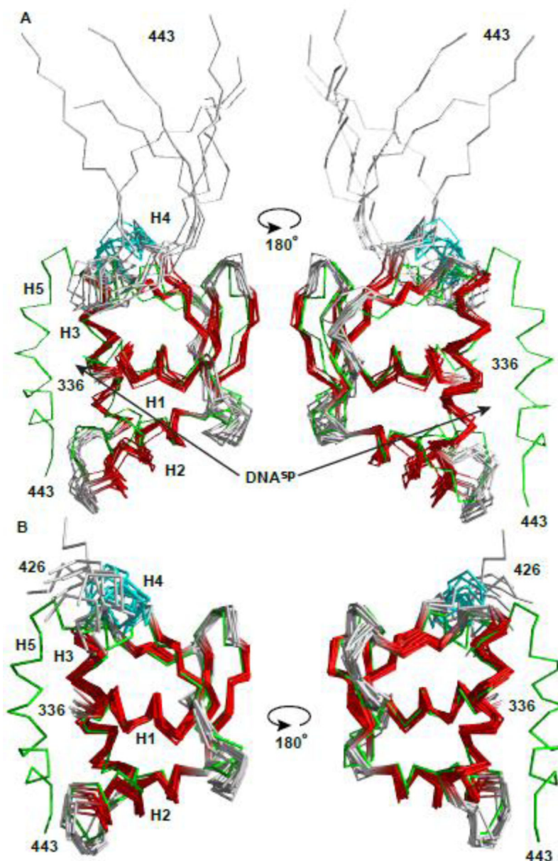
Fig. 3. Structural ensembles of free and bound ETV6 are similar except for the unfolding of helix H5
