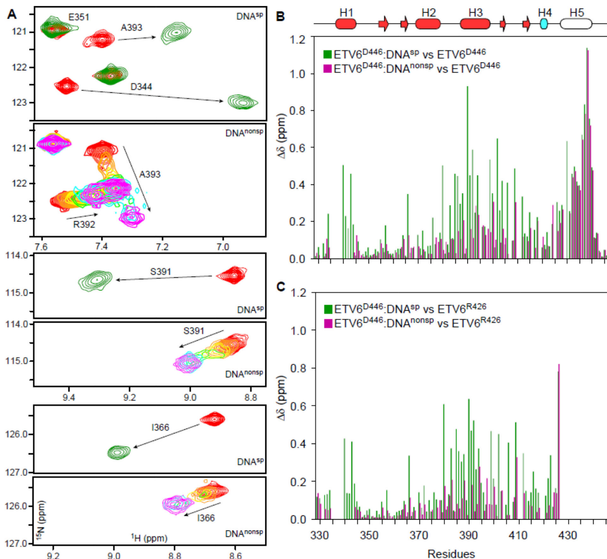
Fig. 1. NMR monitored titrations of ETV6 fragments with DNA
