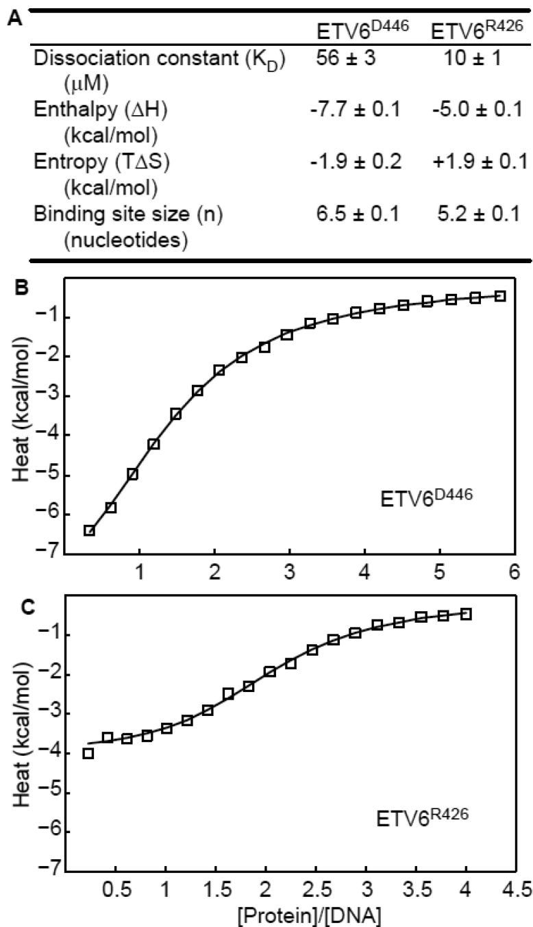
Fig. 4. Binding to non-specific DNA is also auto-inhibited
