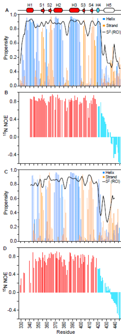
Fig. 2. Helix H5 is unstructured in both specific and non-specific ETV6–DNA complexes The normalized secondary structure propensities (helices, blue; strands, orange) and RCI order parameters ( S^2 , black line) for the (A) ETV6 D446 –DNA sp and (C) ETV6 D446 –DNA nonsp complexes were calculated from ^{13}\text{C}^\alpha , ^{13}\text{C}^\beta , ^{15}\text{N} and ^1\text{H}^\text{N} chemical shifts using the program MICS 81 . The ^{15}\text{N} -NOE data for (B) ETV6 D446 –DNA sp and (D) ETV6 D446 –DNA nonsp are shown for the core ETS domain (red) and CID (cyan) residues. Decreasing NOE and S^2 values indicate increasing amide mobility on the sub-nsec timescale and thus show that helix H5 is unfolded in both complexes (see also Supplemental Fig. S2). The
