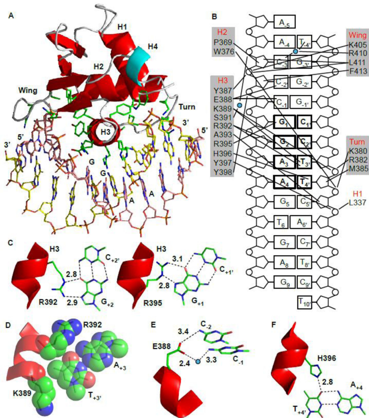
Fig. 6. Binding interface of ETV6 R426 -DNA sp -cryst complex (A) Crystal structure of the ETV6 R426 -DNA sp -cryst complex. ETS domain residues contacting the DNA are shown in stick representation. Secondary structural elements in the core ETS domain are colored red, loops in grey, and helix H4 in cyan. Corresponding backbone atoms for ordered residues in the crystal ETV6 R426 -DNA sp -cryst and solution ETV6 R426 -DNA sp complexes superimposed with an average rmsd of 1.0 Å (not shown). (B) Interfacial interactions with ETV6 residues grouped according to their secondary structure. Water molecules are denoted as blue circles. (C) Direct readout due to the invariant Arg392
