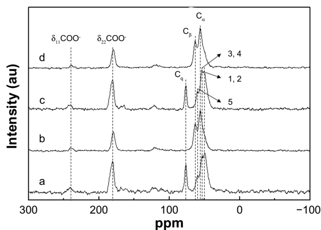
Figure 4 13 C nuclear magnetic resonance results for (a) ZnO SM20(-) , (b) ZnO SM20(+) , (c) ZnO AE100(-) , and (d) ZnO AE100(+) .
