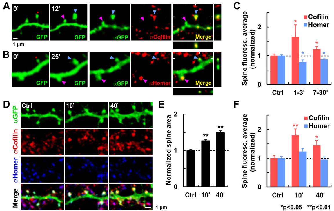
Fig. 3. Redistribution of endogenous cofilin-1 and Homer1b during sLTP
