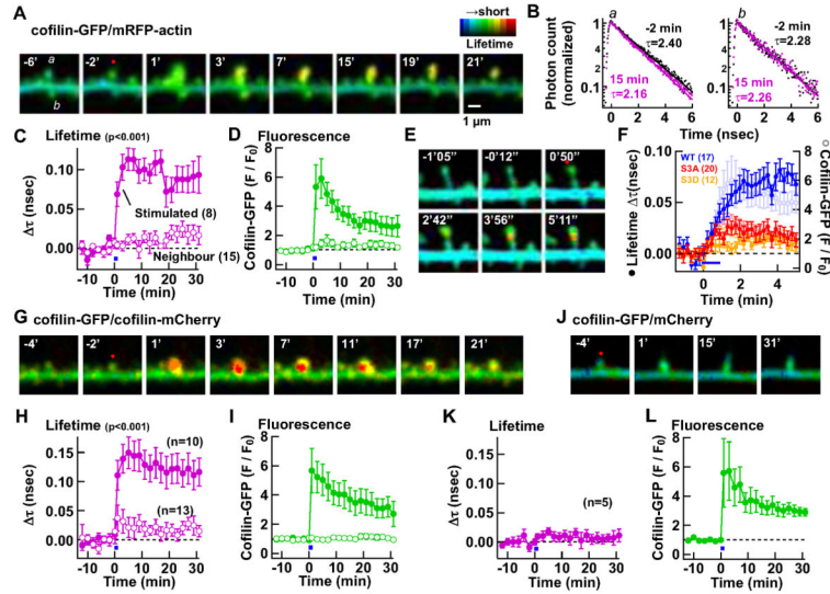
Fig. 5. Cofilin stably interacts with F-actin at a high stoichiometric ratio (A–F) Interaction between cofilin and actin was monitored by FRET-FLIM between cofilin-GFP and mRFP-actin. (A) Representative time-lapse FLIM images. sLTP was induced in spine a (red dot) between 0–1 min. (B) Fluorescence lifetime ( \tau ) of the stimulated spine a (left) and an unstimulated spine b (right) before (black) and 15 min after sLTP induction (pink). (C–D) Time course of averaged changes in lifetime (C) and amount of cofilin-GFP (D) in stimulated and neighboring spines (mean \pm SEM). Number of spines in parenthesis. (E) Faster time course images where only one optical section was monitored. (F) Summary of data similar to E , showing time course of changes in lifetime (filled circles) and amount of cofilin-GFP (open circles) for WT-cofilin, S3A and S3D cofilin mutants. (G–I) A similar experiment to identify the proximity between cofilin molecules by detecting FRET-FLIM between cofilin-GFP and cofilin-mCherry. (J–L) A negative control experiment with cofilin-GFP and free mCherry. See also Fig. S4.
