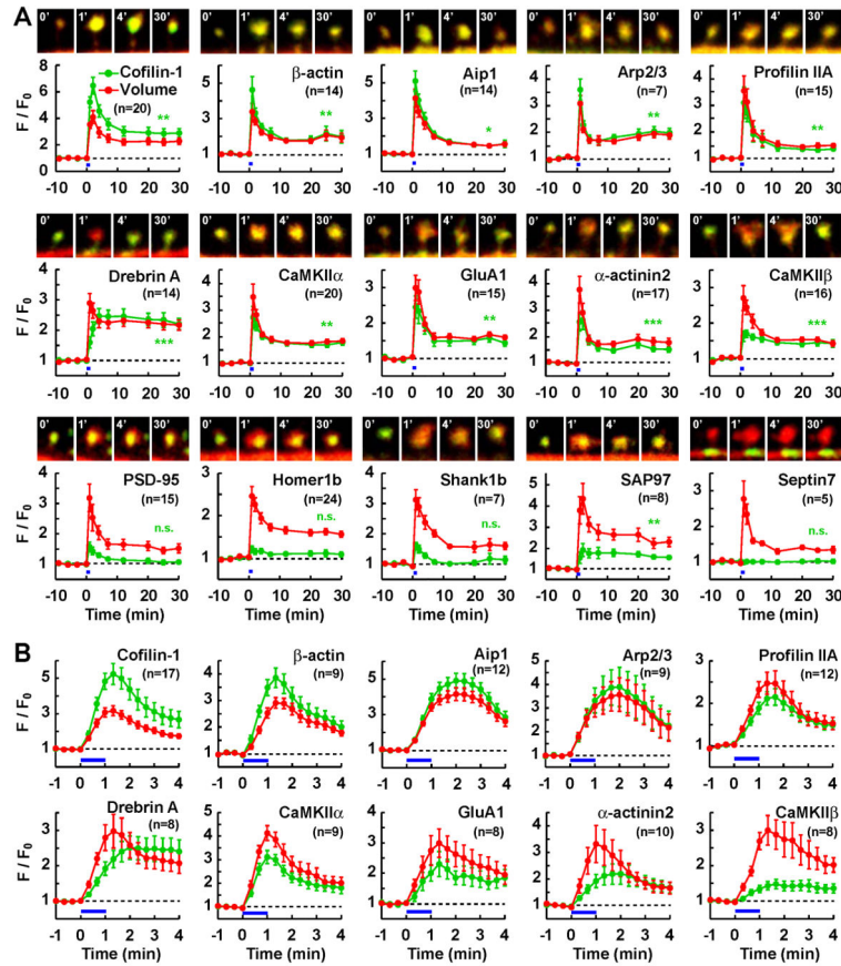
Fig. 1. Diverse temporal patterns of postsynaptic protein translocation to the dendritic spine during sLTP
