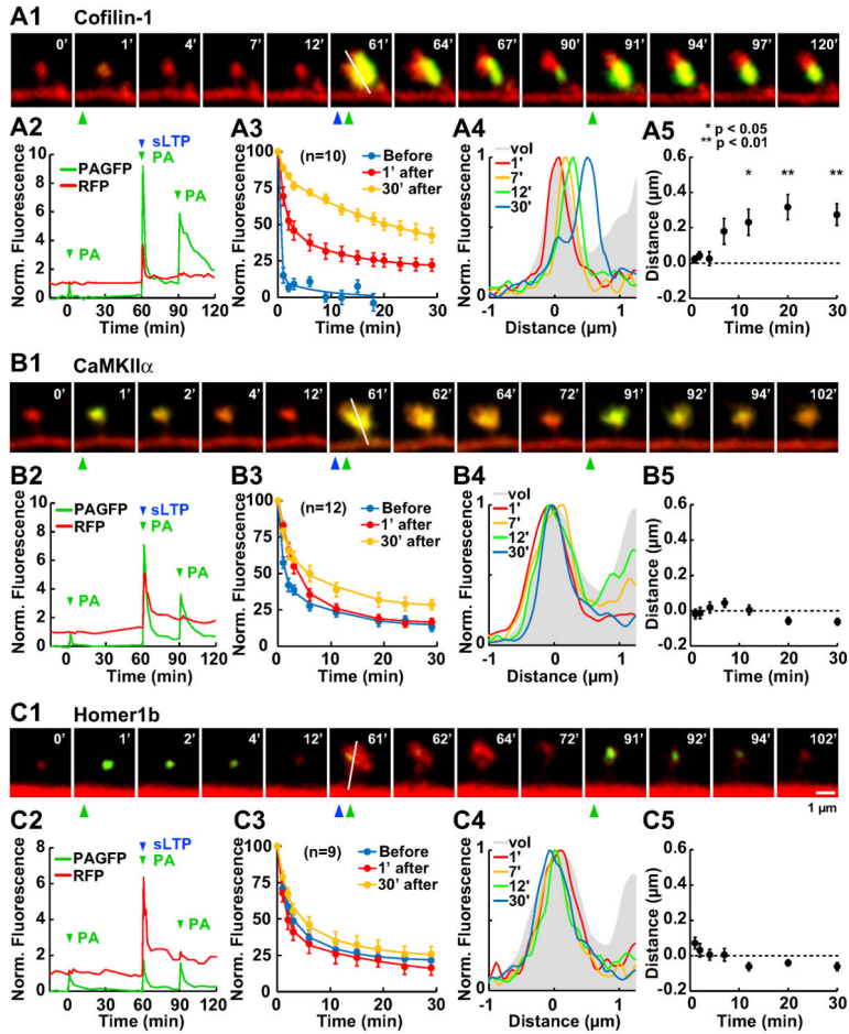
Fig. 4. Persistent changes in protein turnover after single spine sLTP induction
