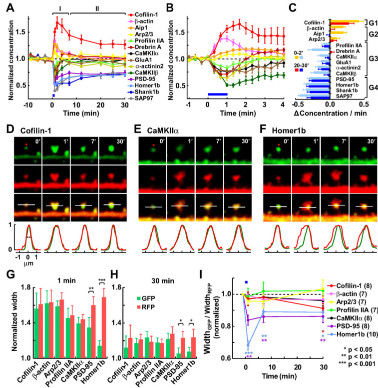
Fig. 2. Changes in spine concentration and subspine distribution of postsynaptic proteins during sLTP
