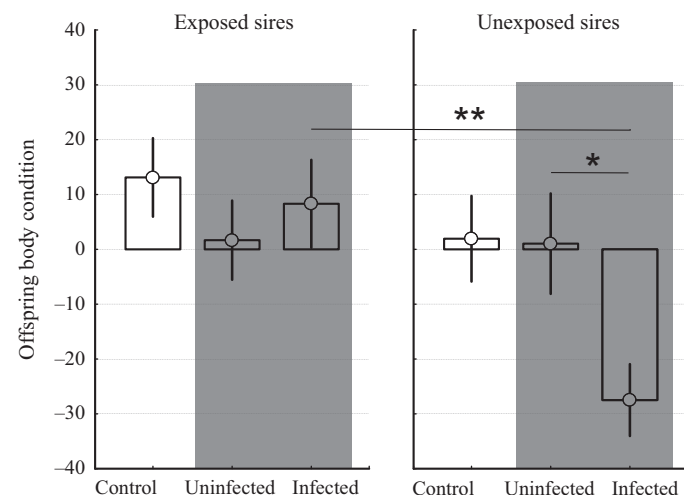
Figure 3 Transgenerational effects of paternal parasite exposure on body condition at the end of the experiment. Body condition is an estimate of fish health and is calculated using the residuals from the regression of body mass on body length. Shown are the means of body condition in control, uninfected (i.e. exposed but non-infected) and infected offspring, sired by either exposed or unexposed fathers. Error bars represent \pm 1 SE. The shaded data indicates the comparison of exposed-uninfected and exposed-infected fish. Symbols represent significant differences between experimental groups based on Tukey post hoc tests (* P = 0.048 ; ** P = 0.003 ).
