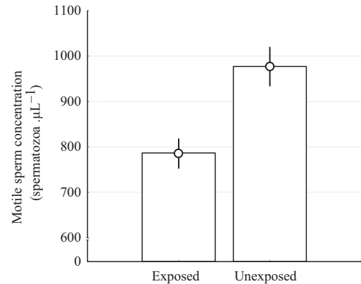
Figure 1 Parasite infection induces sperm deficiency. Concentration of motile spermatozoa per \mu\text{L} in male sticklebacks experimentally infected with the nematode Camallanus lacustris and in uninfected (unexposed) males. Error bars represent \pm 1 SE.
