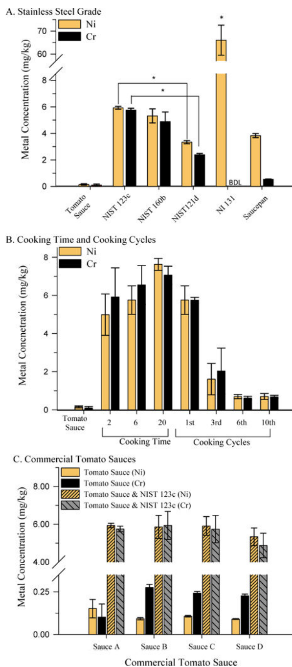
Figure 1. Metal Released from Stainless Steel into Tomato Sauce
