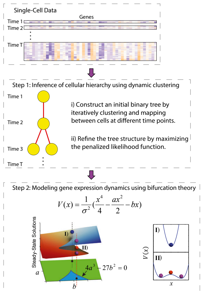
Fig. 1. Overview of the SCUBA method. ( Top ) Structure of single-cell data. Individual cell samples are ordered by their corresponding developmental time. ( Middle and Bottom ) Schematic of the two main steps of SCUBA. In the bottom panel, the parameter space is divided into two regions, corresponding to one (green region and I) or two attractor states (blue region and II), respectively. The surface on top of parameter space shows the steady-state solutions corresponding to each parameter setting. Stable and unstable steady states are colored differently.
