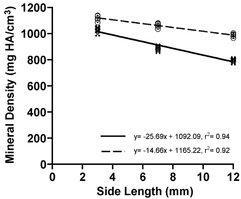
Figure 5. Bivariate plot of tissue mineral density ( \rho_m ) and bovine cortical bone (BCt) cube side length. Solid line (with dark cross symbols) represents data processed with the 200 mg HA/cm 3 BHC and the dashed line (with open circles) represents data processed with the 1200 mg HA/cm 3 BHC.
