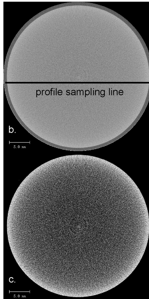
Figure 6. Micro-computed tomography images (0.036 mm isotropic voxels) demonstrating the cupping artifact in a liquid dipostassium phosphate phantom. The grayscale intensity profile (a) of the original image (b) confirms the presence of the cupping artifact characterized by radial decreases in the grayscale intensity from the periphery towards the center. Although the grayscale changes appear subtle to the naked eye, the grayscale values in the center of the image are approximately 17% lower than the values along the outer limit of the phantom. Reduction of the image's grayscale dynamic range (c) visually reinforces the pixel
