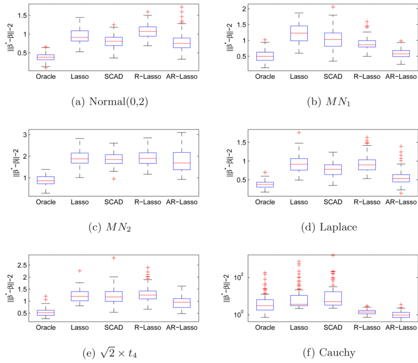
Fig. 1. Boxplots for L_2 Loss with Correlated Covariates
