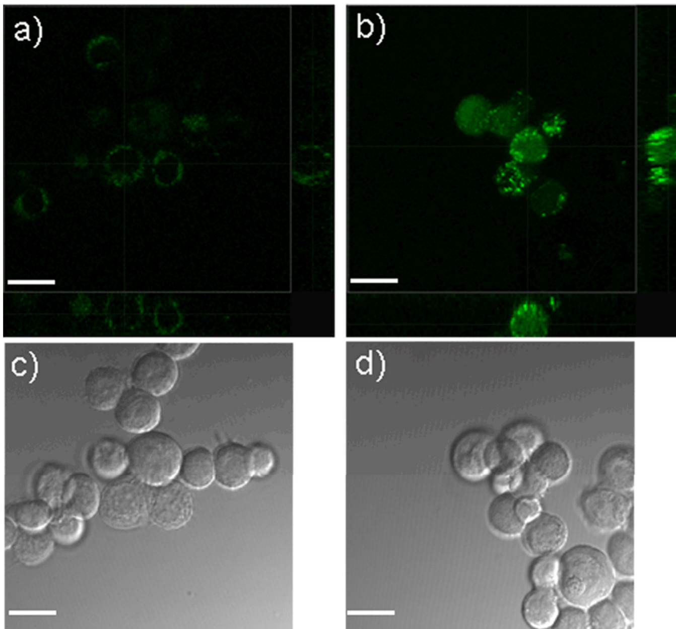
Fig. 3. Internalization of peptides into MCF7 cells in vitro . MCF cells are incubated with lin-R 4 F 2 -FITC (a, c) or cyc-R 4 F 2 -FITC (b, d) at 10 \mu M concentration for 5 hrs without serum. a), b): three-dimensional reconstructions of the LSCM images of cells after incubation with lin-R 4 F 2 -FITC (green) and cyc-R 4 F 2 -FITC (green), respectively, showing greater internalization for the latter case; c), d): the corresponding differential interference contrast images of a), b) (Scale bar = 40 \mu m).
