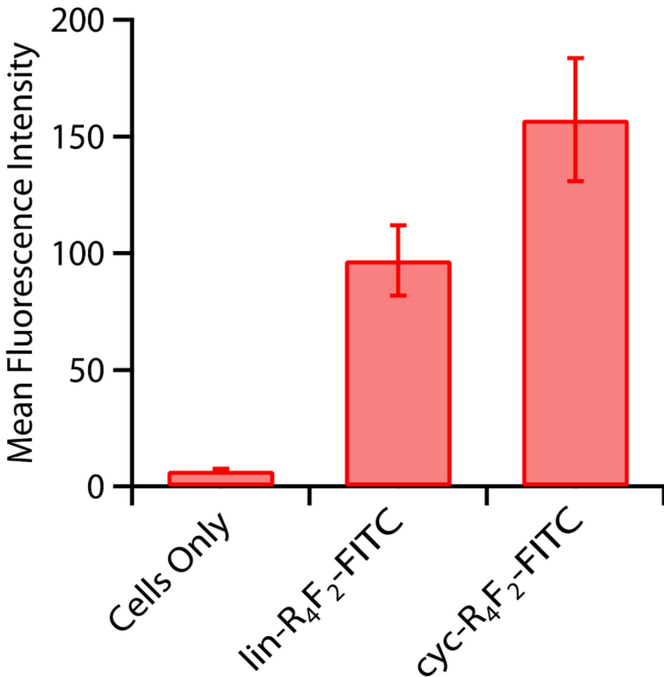
Fig. 4. FACS analysis showing quantitative uptake of peptides into MCF7 cells, showing the progressive increase from incorporation of peptide hydrophobicity and cyclicality. Cells are incubated with 5 \mu M peptides for 5 hrs without serum. Error bars represent standard errors of the mean.
