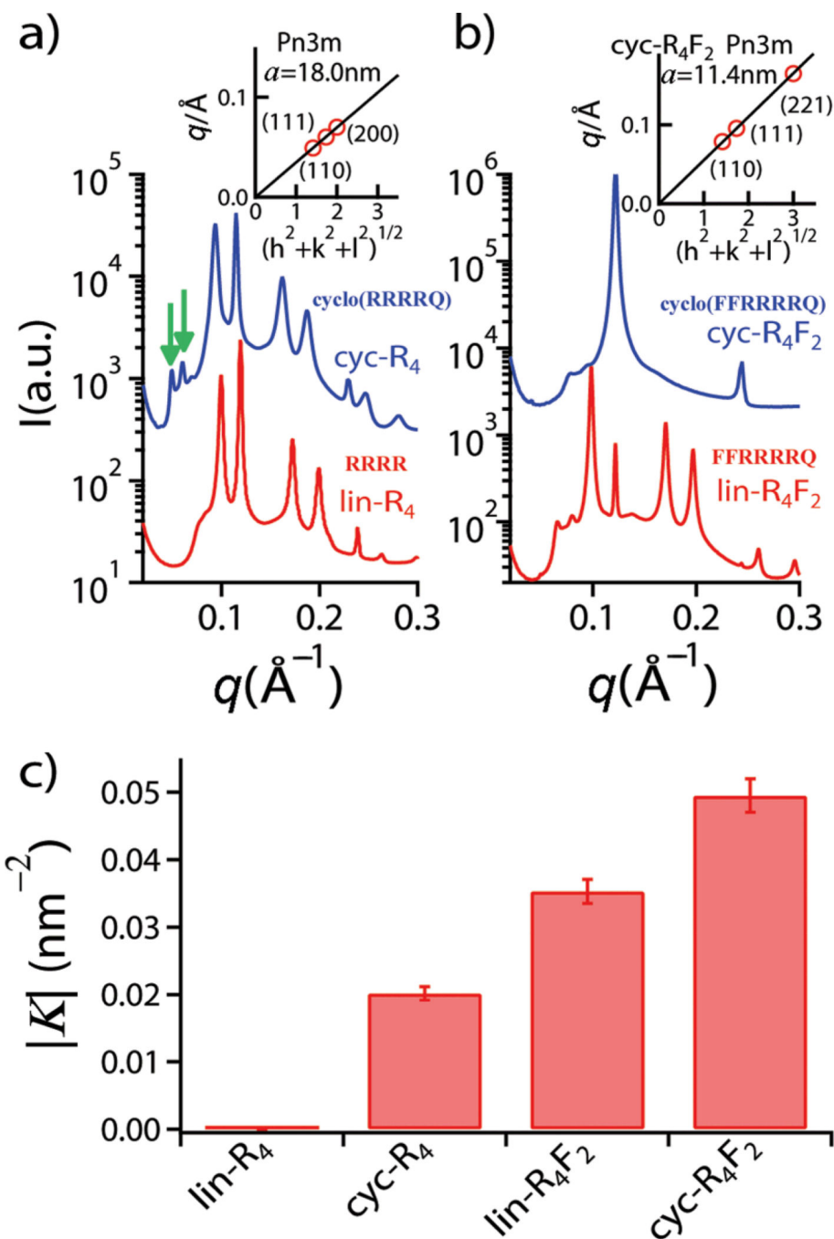
Fig. 1. Comparison between cyclic peptides ( \text{cyc-R}_4 , \text{cyc-R}_4\text{F}_2 ) and their linear counterparts ( \text{lin-R}_4 , \text{lin-R}_4\text{F}_2 ). a) SAXS measurement for \text{cyc-R}_4 and \text{lin-R}_4 ; b) SAXS measurement for \text{cyc-R}_4\text{F}_2 and \text{lin-R}_4\text{F}_2 (DOPS/DOPE/DOPC = 20/80/00, peptide/lipid molar ratio P/L = 1/10). The SAXS intensity curves in a) and b) are shifted for clarity. c) Calculated average magnitude of Gaussian curvature |K| from the lattice constants of Pn3m cubic phase. Insets in a) and b) show indexing of the Pn3m cubic phase by agreement between the measured peak q positions and the Miller indices h, k, l , with relationship q = 2\pi(h^2+k^2+l^2)^{1/2}/a , for a
