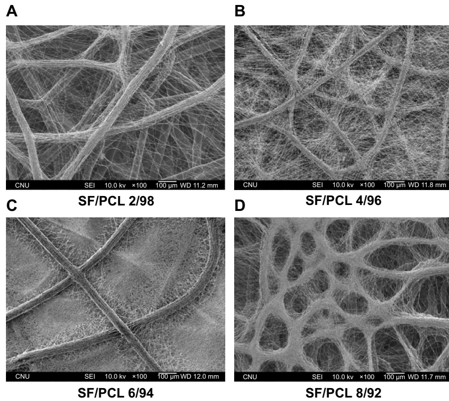
Figure S2 Changes in morphology of water vapor-treated SF/PCL nano/microfibrous composite scaffolds after water immersion for 1 hour. Notes: (A) SF/PCL 2/98, (B) SF/PCL 4/96, (C) SF/PCL 6/94, and (D) SF/PCL 8/92. Abbreviations: PCL, poly( \epsilon -caprolactone); SF, silk fibroin.
