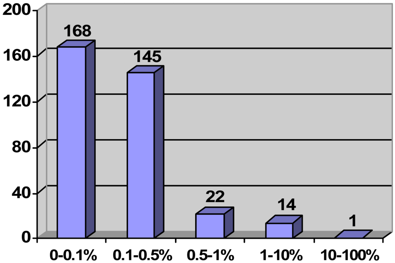
Figure 1. Frequency distribution of pattern pairs
